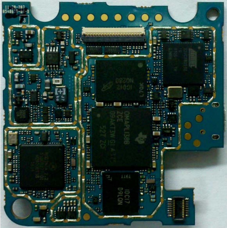
RF board without Shields (Top)
