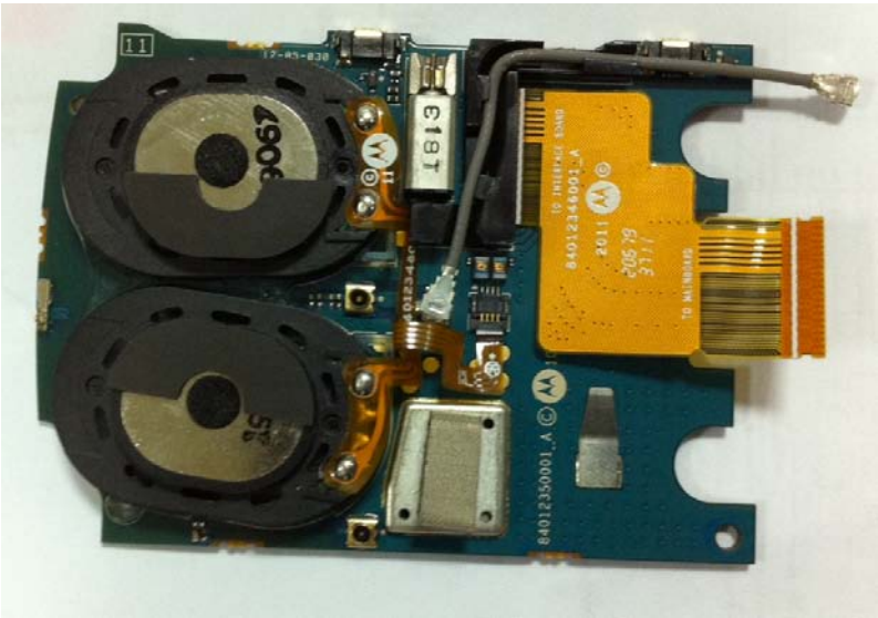
Interface board with Shields (Top)
