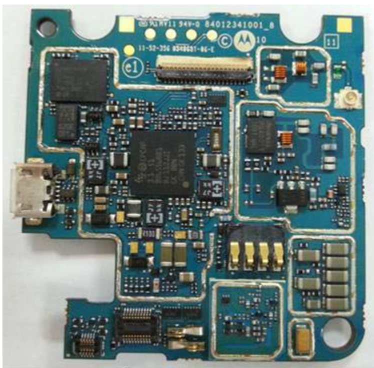
RF board without Shields (Bottom)
