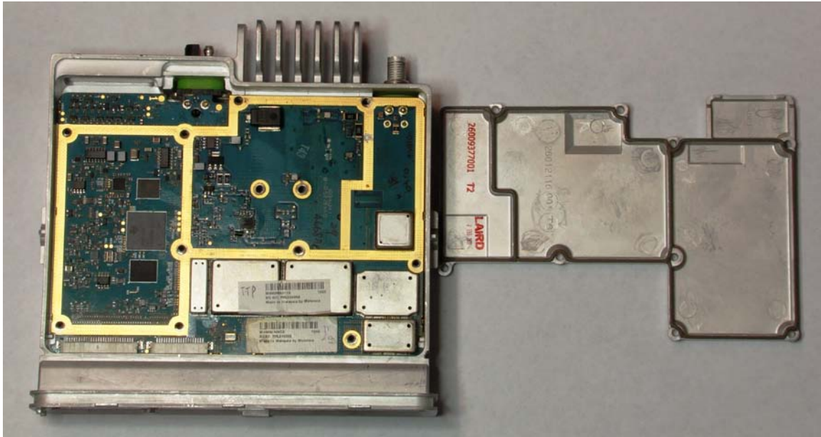
TOP VIEW WITH CHASSIS TOP COVER REMOVED (MATING SURFACES OF TOP COVER AND CIRCUIT BOARD IN CHASSIS ARE SHOWN)
