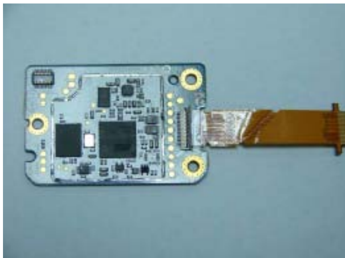
GOB board without shields (Top)
