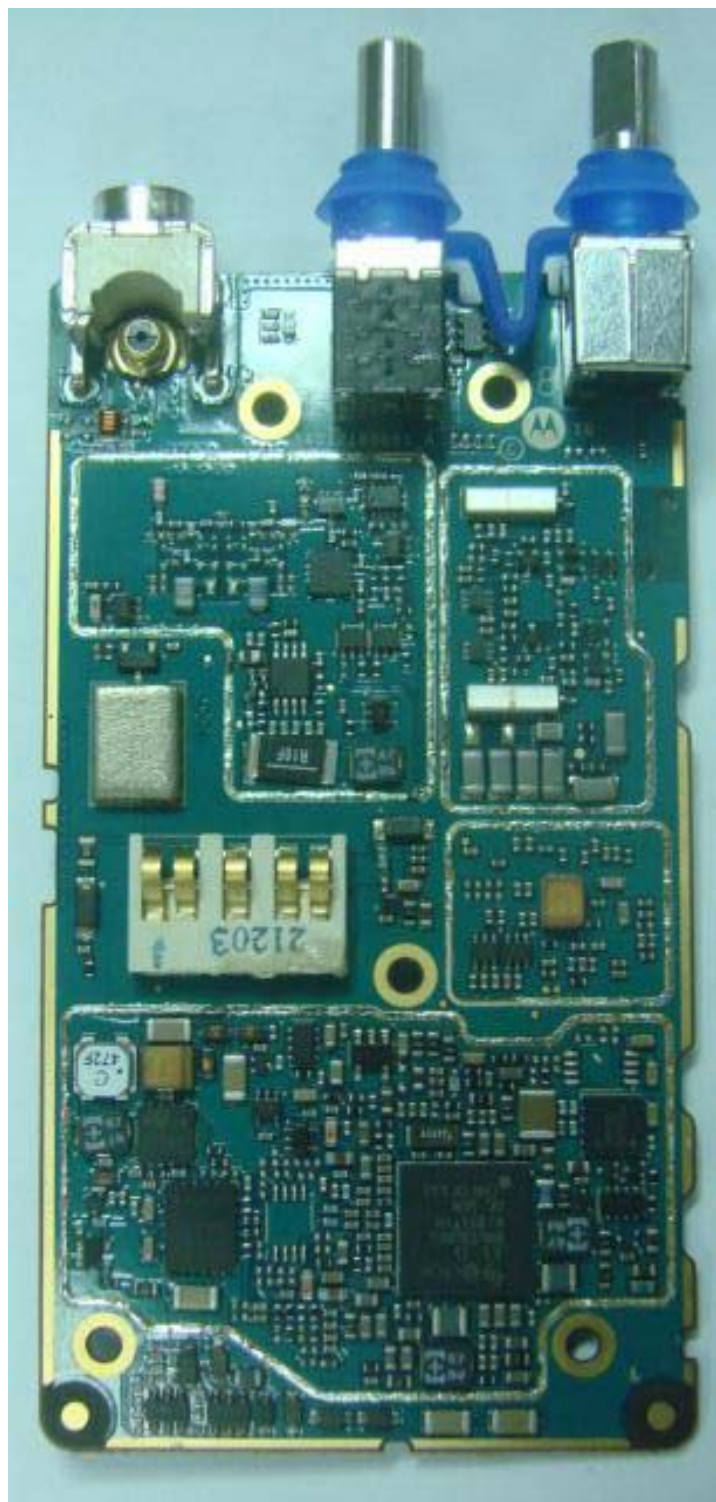
RF board without Shields (Bottom)
