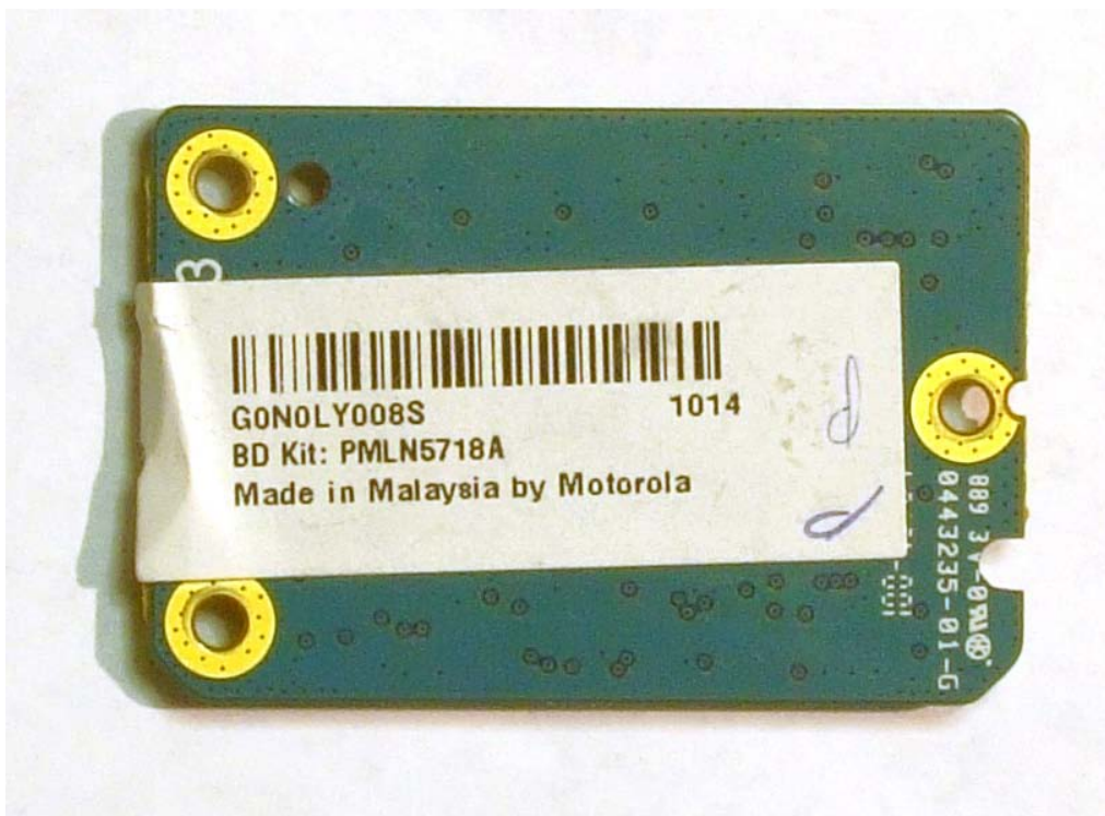
FRONT VIEW OF BLUETOOTH/GPS BOARD
