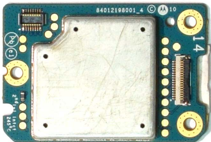
BACK VIEW OF BLUETOOTH/GPS BOARD
