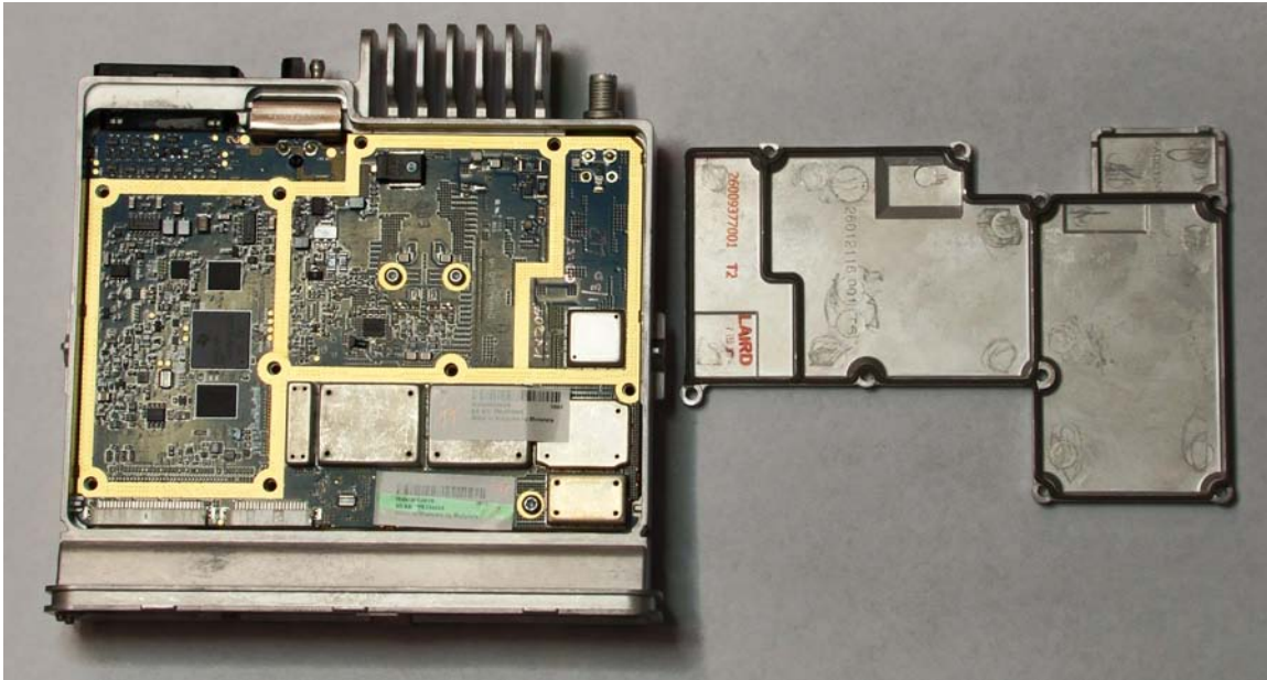
TOP VIEW WITH CHASSIS TOP COVER REMOVED (MATING SURFACES OF TOP COVER AND CIRCUIT BOARD IN CHASSIS ARE SHOWN)
