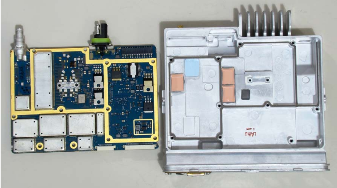
TOP VIEW WITH CIRCUIT BOARD REMOVED FROM CHASSIS (MATING SURFACES OF CIRCUIT BOARD AND CHASSIS ARE SHOWN)
