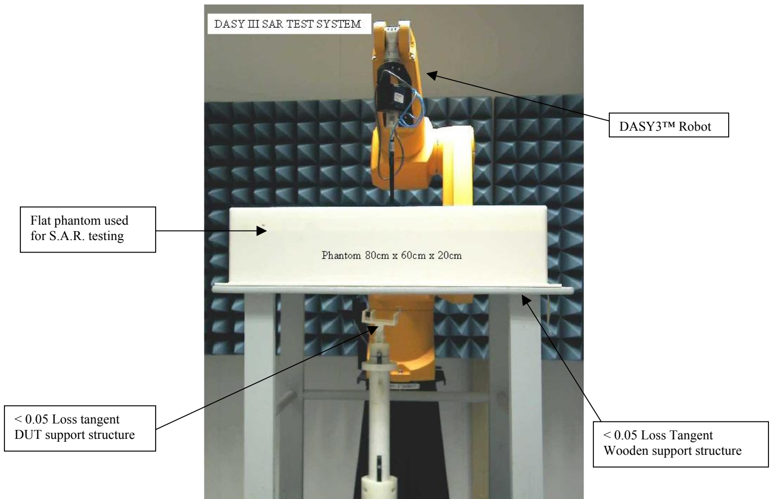
Figure 2: Robot Test System
