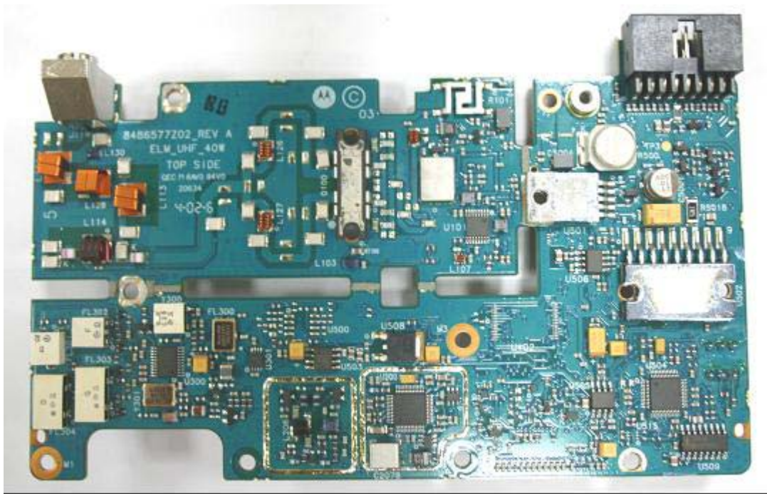
Figure 9-1: Top Side of PCB without shields.
