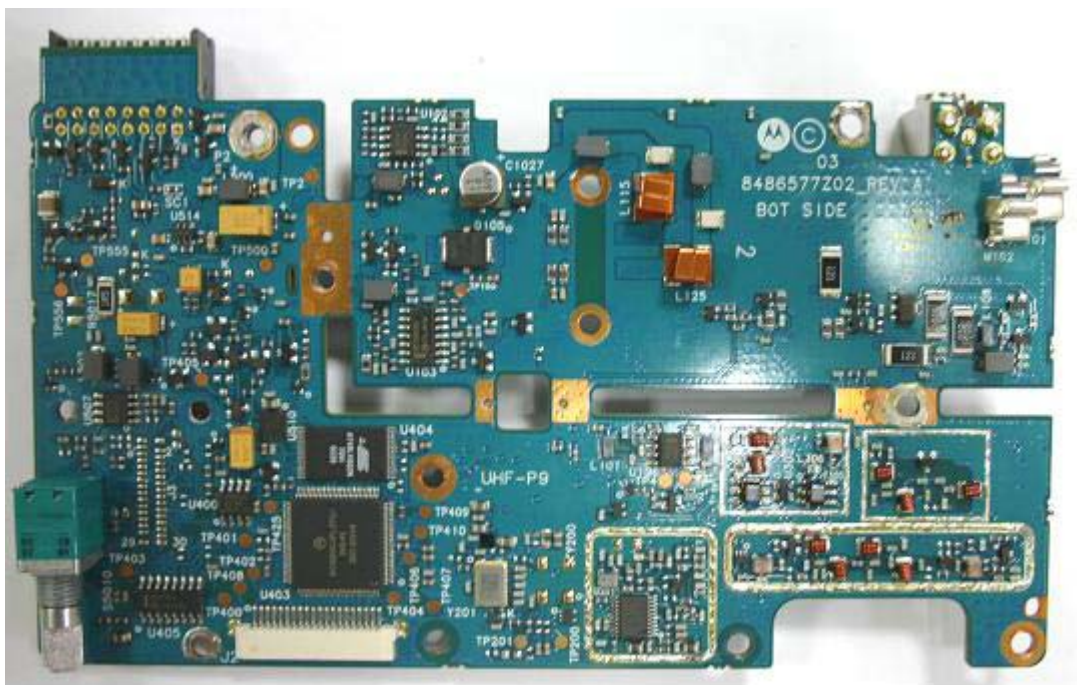
Figure 9-2: Bottom Side of PCB without shields.
