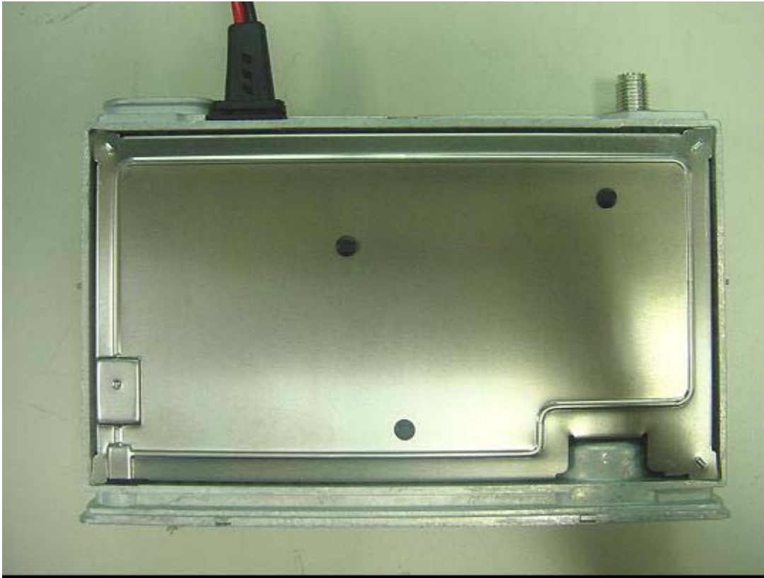
Figure 9-7: Top view of chassis with main shield in place.
