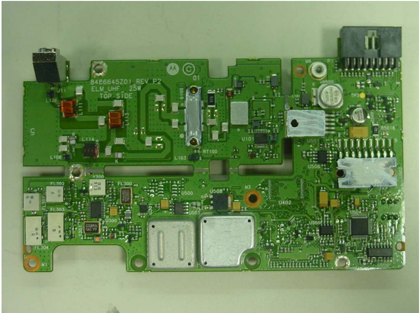
Figure 9-1: Top Side of PCB with shields.
