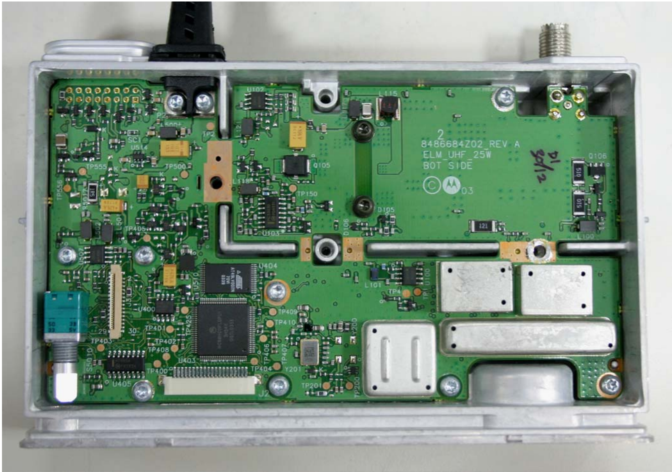
Figure 9-3: Top View of PCB placed in chassis.
