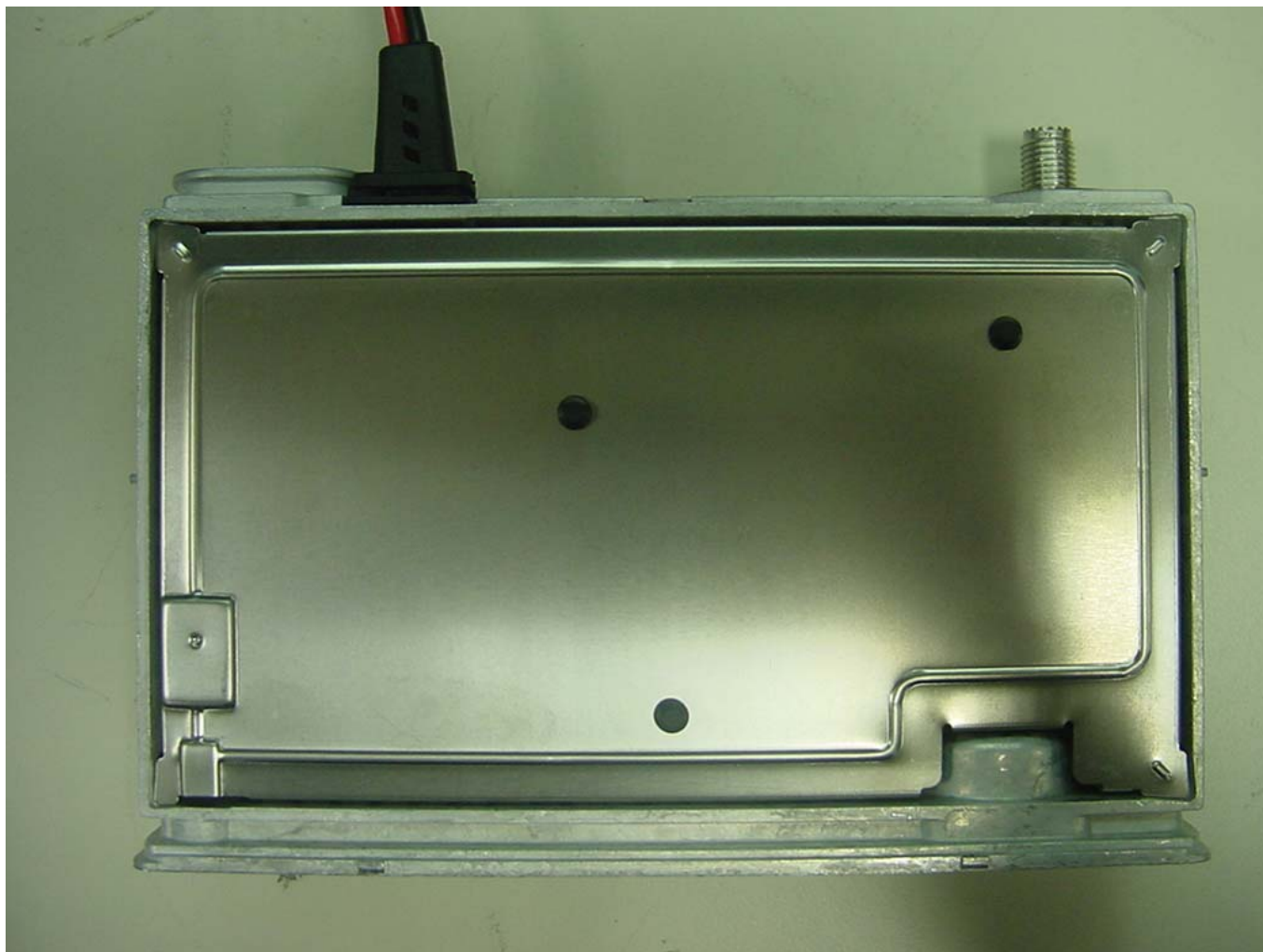
Figure 9-5: Top view of chassis with main shield in place.
