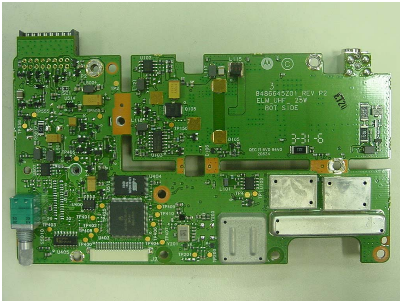
Figure 9-2: Bottom Side of PCB with shields.
