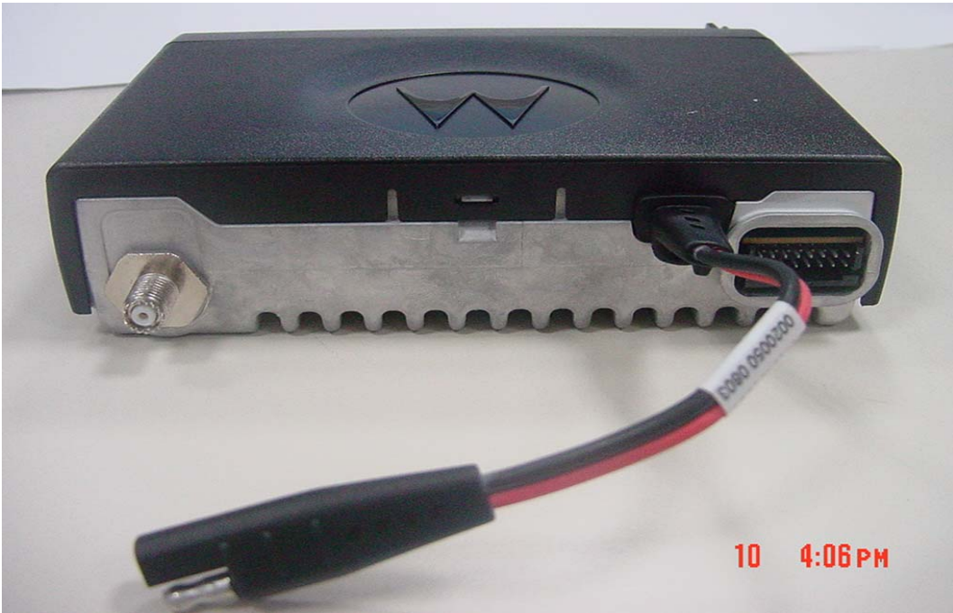
Figure 3-3: Rear view of complete radio showing antenna connector, DC cable, and accessory connector.
