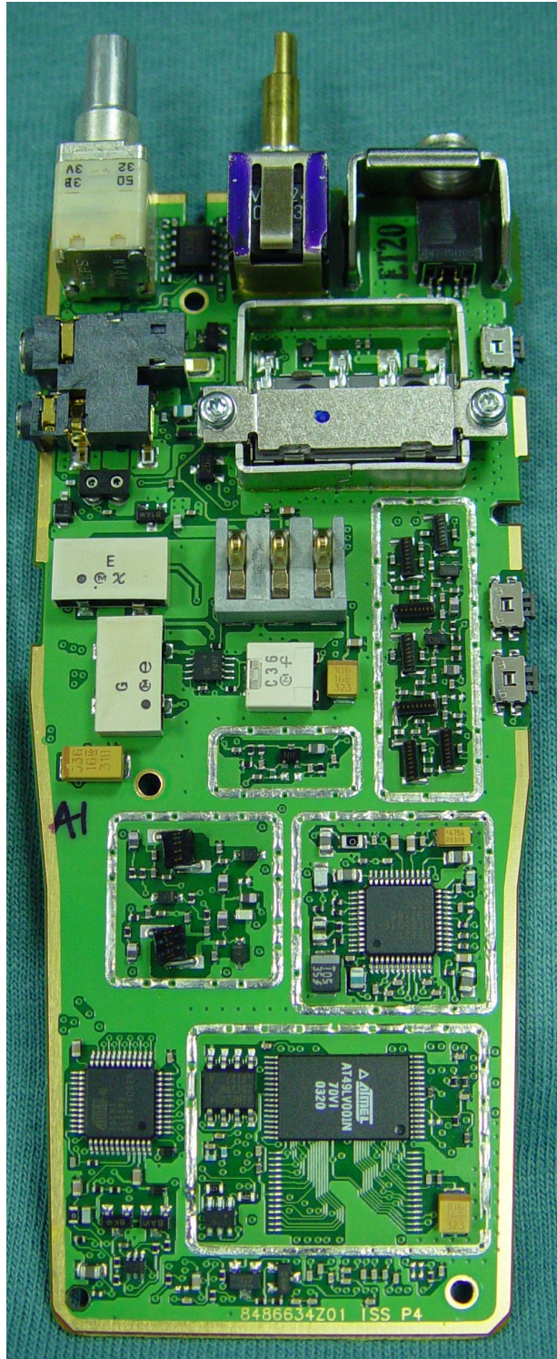
REAR VIEW OF CIRCUIT BOARD WITH ALL SHIELDS REMOVED
