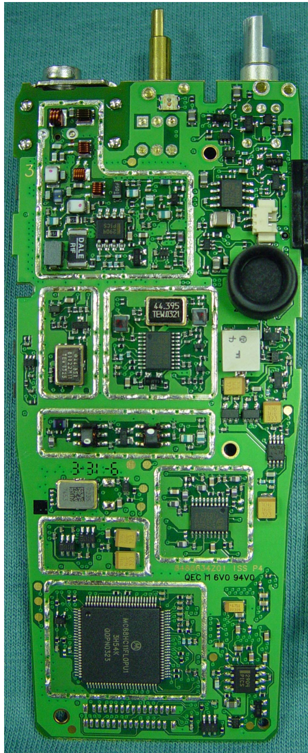
FRONT VIEW OF CIRCUIT BOARD WITH ALL SHIELDS REMOVED
