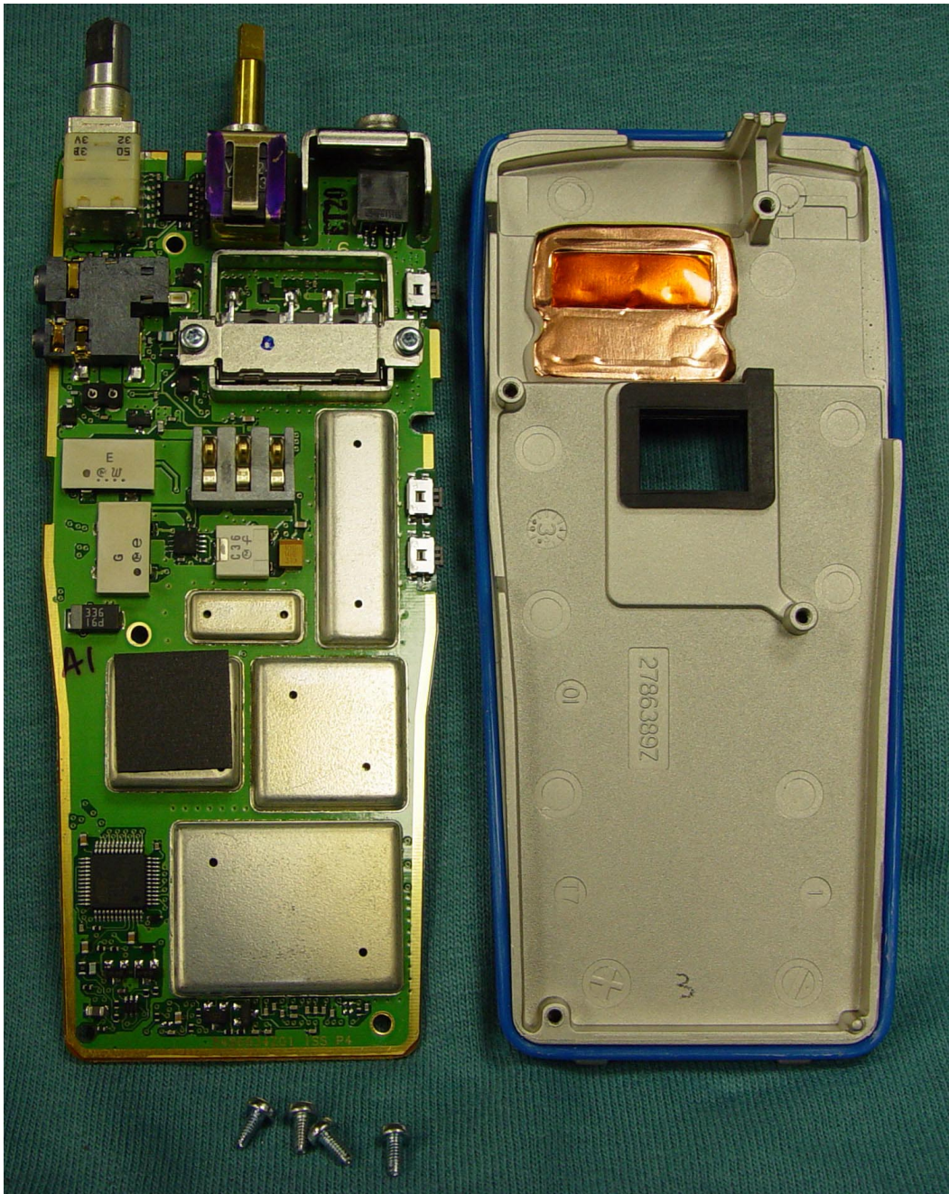
REAR VIEW OF CIRCUIT BOARD REMOVED FROM CHASSIS (MATING SURFACES OF CIRCUIT BOARD AND CHASSIS ARE SHOWN)
