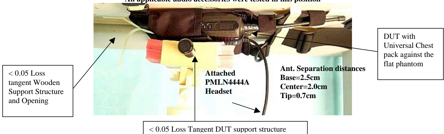
Figure 1: Highest S.A.R. Test Position (DUT with Universal Chest Pack model HLN6602A against the flat phantom w/ attached headset model PMLN4444A) All applicable audio accessories were tested in this position
