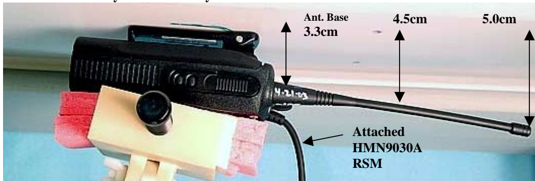
Figure 3. Assessment @ the Abdomen; DUT w/ body worn accessory model HLN8255 and attached HMN9030A RSM
