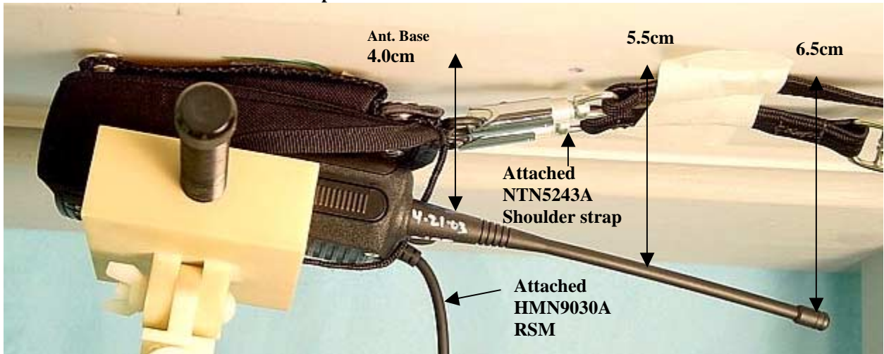
Figure 2. Assessment @ the Abdomen; DUT w/ body worn accessory model HLN9701B W/ attached shoulder strap and model NTN5243A and attached HMN9030A RSM
