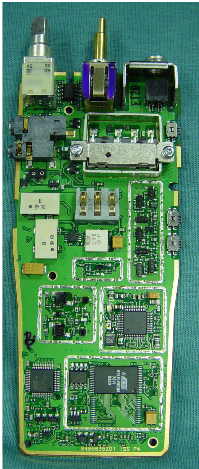
REAR VIEW OF CIRCUIT BOARD WITH ALL SHIELDS REMOVED
