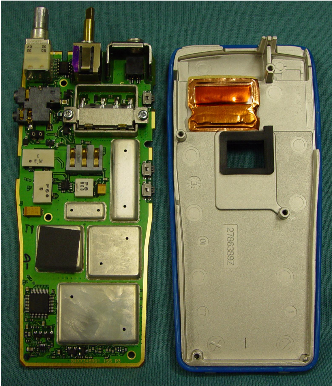
REAR VIEW OF CIRCUIT BOARD REMOVED FROM CHASSIS (MATING SURFACES OF CIRCUIT BOARD AND CHASSIS ARE SHOWN)
