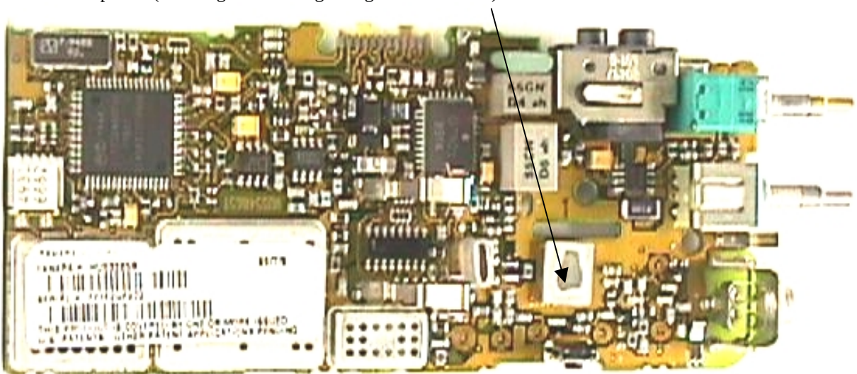
UHF SP50 Top Side (Showing heat-sinking change for MRF1507).
