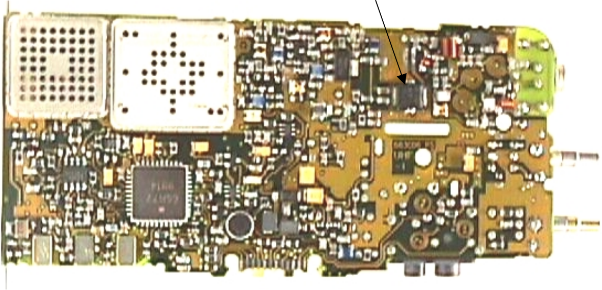
UHF SP50 Bottom Side (Showing MRF1507 transistor and matching circuits).
