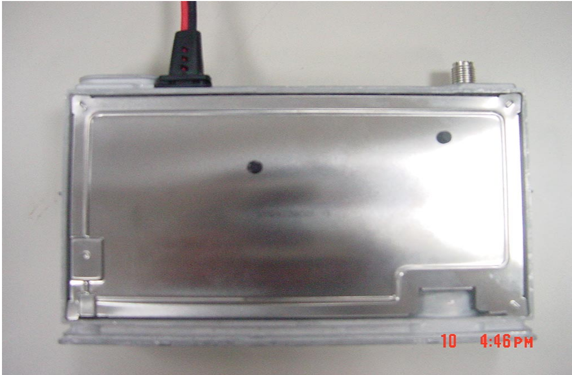
Figure 9-7: Top view of chassis with main shield in place.
