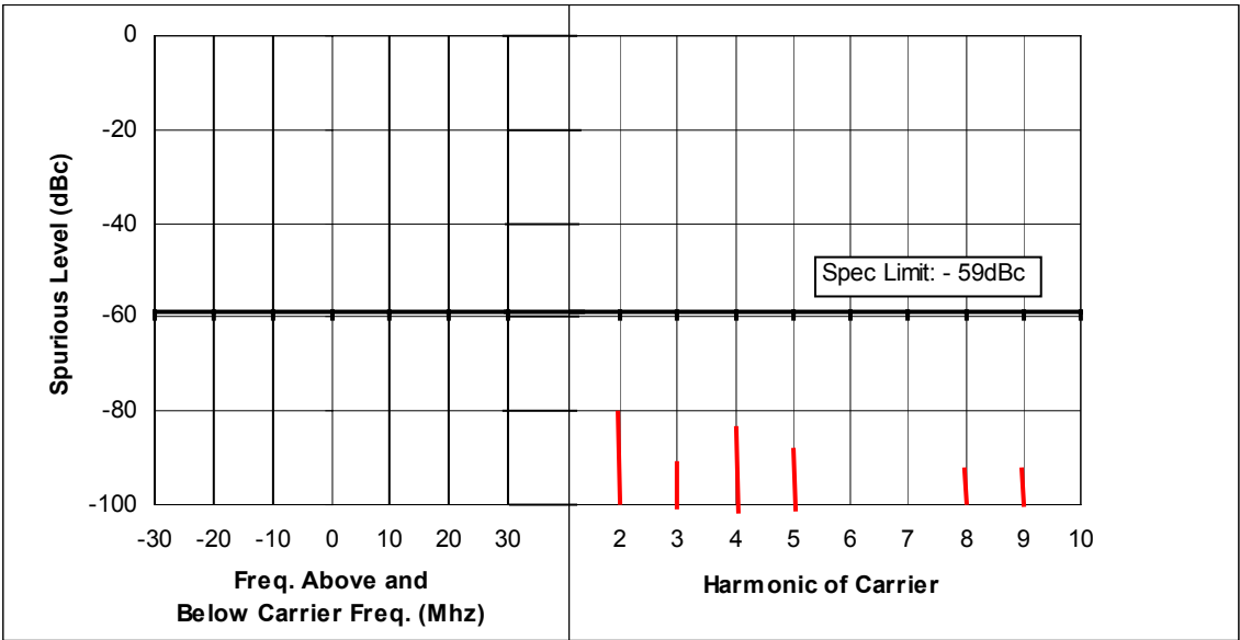
Figure 6F-5: 44 Watts, 454.0125 MHz, 25 kHz Channel Spacing
