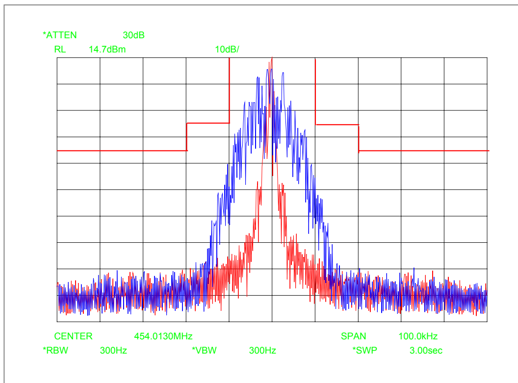
Figure 6E-14: 25 KHz Channel Spacing, 2000/3000 Hz FSK Data and PL Tone Modulation, Mask B
