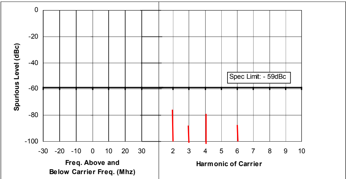
Figure 6F-6: 44 Watts, 469.9875 MHz, 25 kHz Channel Spacing
