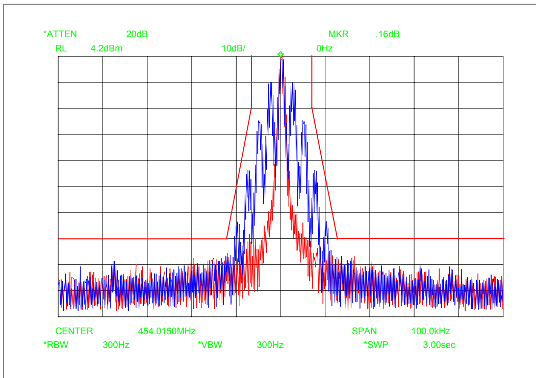
Figure 6E-2: 12.5 KHz Channel Spacing, 2500 Hz Audio and PL Tone Modulation, Mask D
