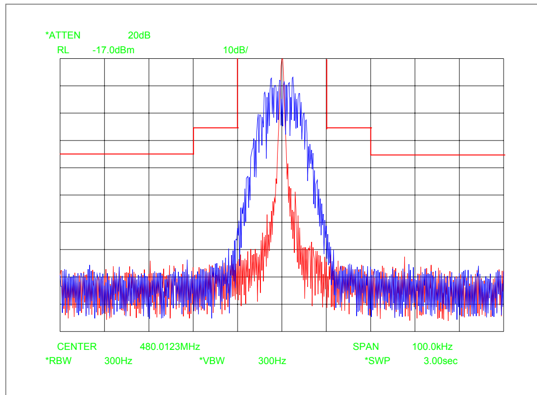
Figure 6E-16: 25 KHz Channel Spacing, DTMF Modulation Only , Mask B
