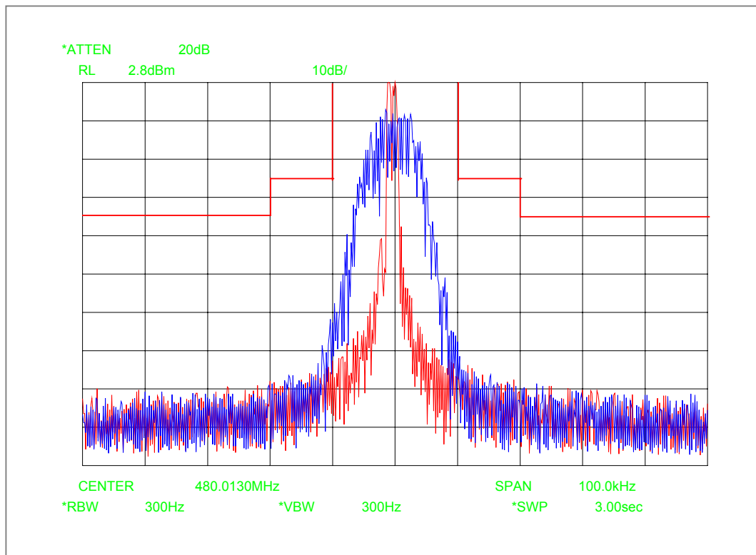
Figure 6E-18: 25 KHz Channel Spacing, DTMF Modulation and DPL Tone Modulation, Mask B
