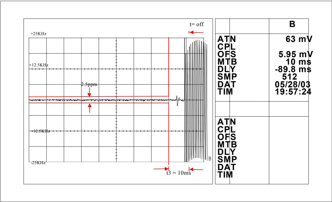
Figure 6I-2: 44 Watts, 12.5 KHz De-Key Decay Time
