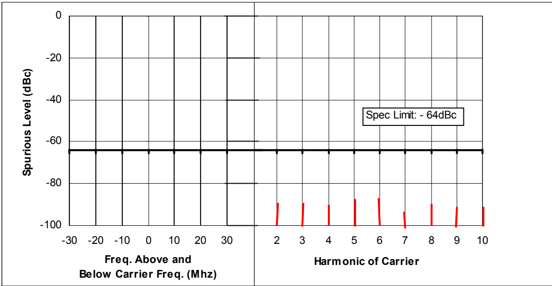
Figure 6F-9: 25 Watts, 469.9875 MHz, 12.5 kHz Channel Spacing
