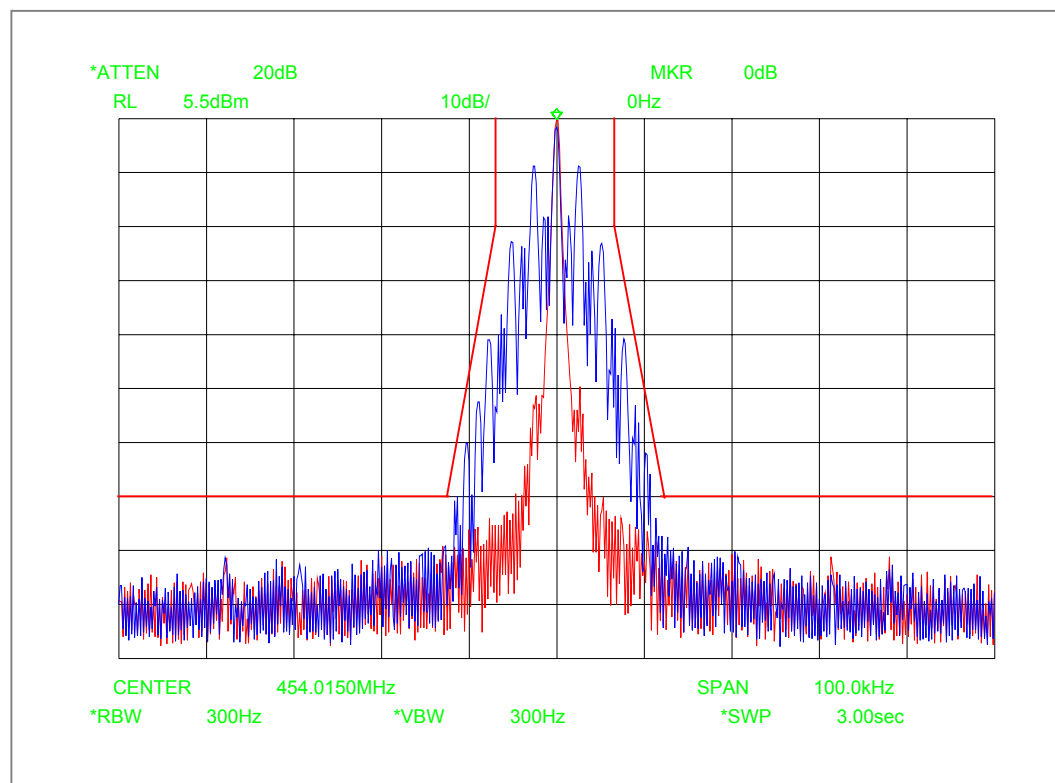
Figure 6E-4: 12.5 KHz Channel Spacing, 2000/3000 Hz FSK Data Modulation Only, Mask D
