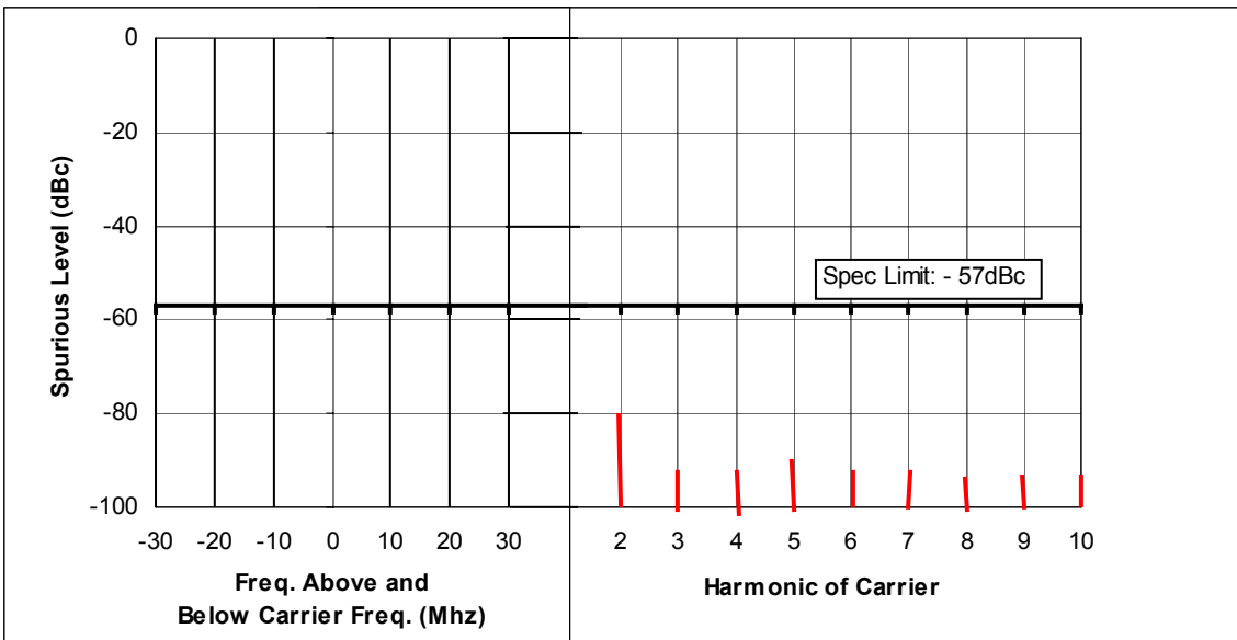
Figure 6F-10: 25 Watts, 438.0125 MHz, 25 kHz Channel Spacing
