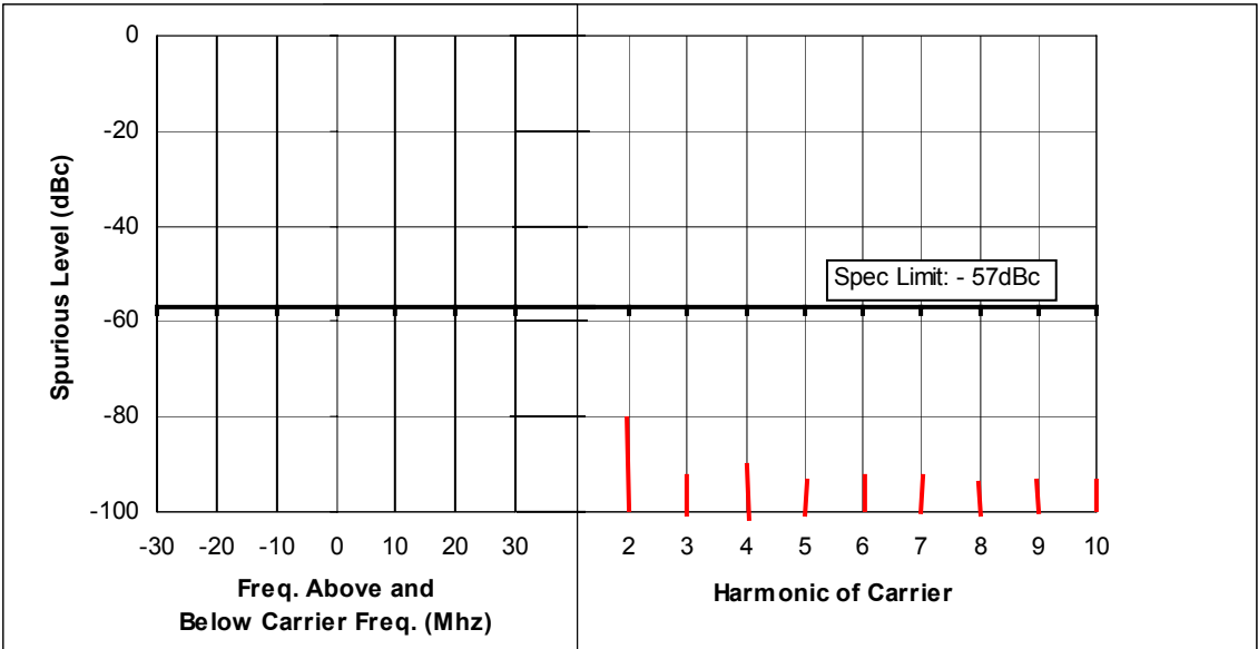
Figure 6F-12: 25 Watts, 469.9875 MHz, 25 kHz Channel Spacing
