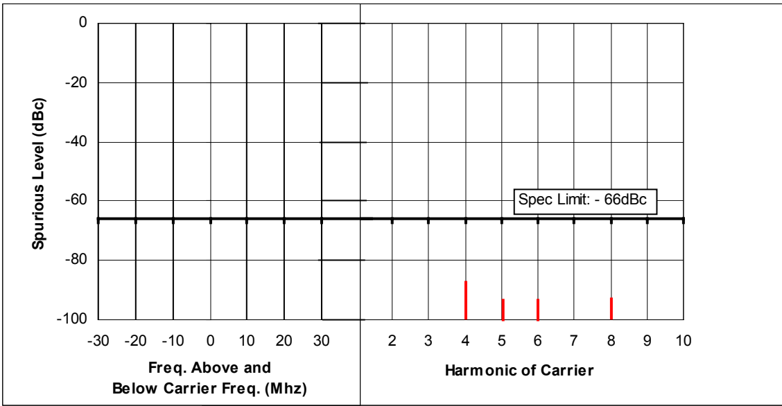
Figure 6F-3: 44 Watts, 469.9875 MHz, 12.5 kHz Channel Spacing
