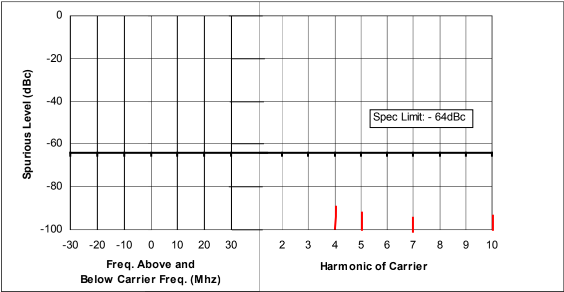
Figure 6F-7: 25 Watts, 438.0125 MHz, 12.5 kHz Channel Spacing
