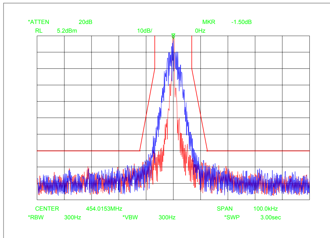
Figure 6E-9: 12.5 KHz Channel Spacing, DTMF Modulation and DPL Tone Modulation , Mask D
