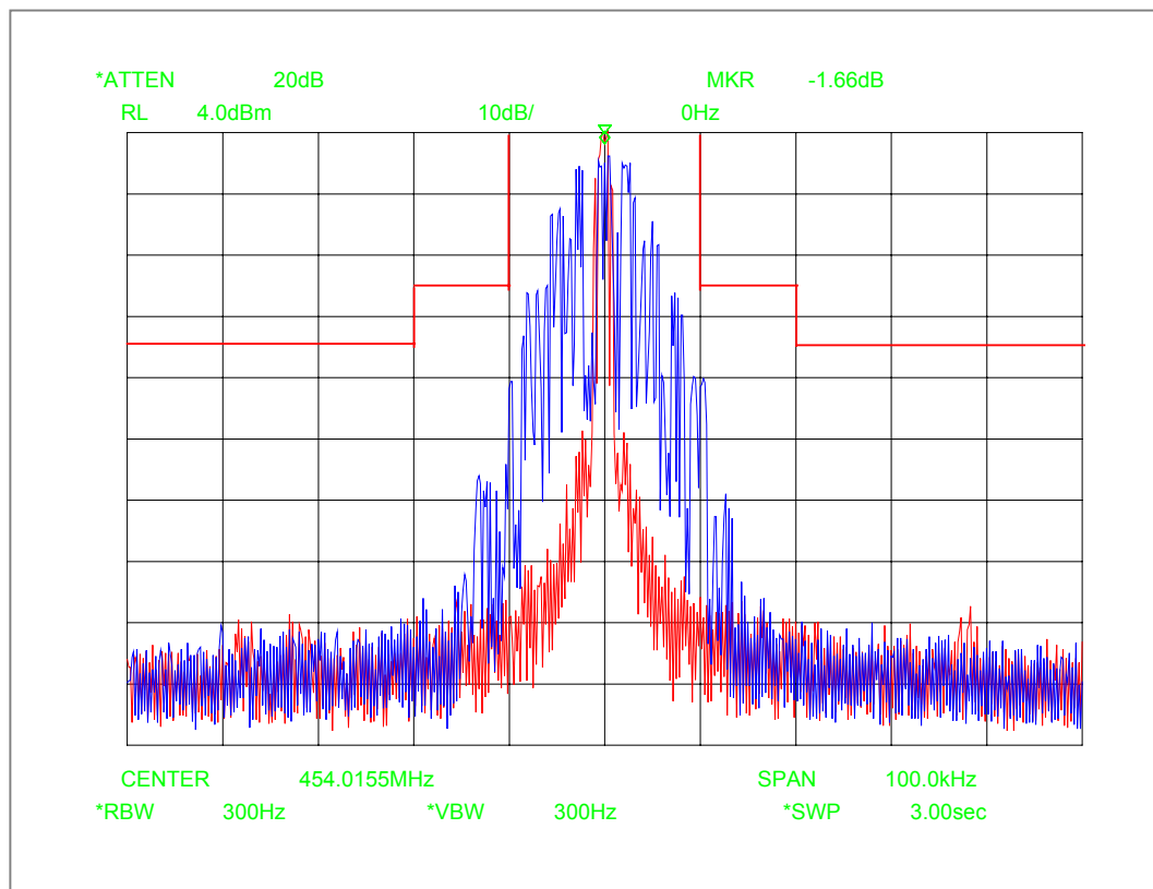
Figure 6E-12: 25 KHz Channel Spacing, 2500 Hz Audio and DPL Tone Modulation, Mask B
