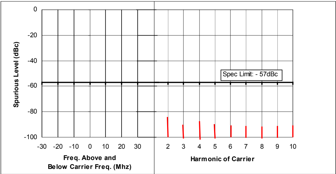
Figure 6F-11: 25 Watts, 454.0125 MHz, 25 kHz Channel Spacing
