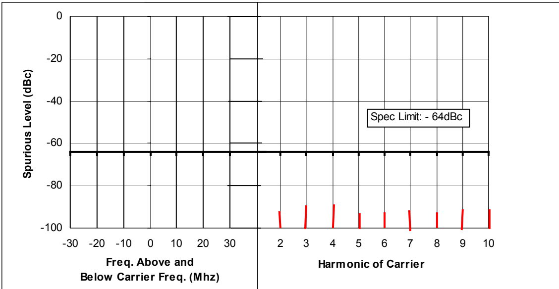
Figure 6F-8: 25 Watts, 454.0125 MHz, 12.5 kHz Channel Spacing
