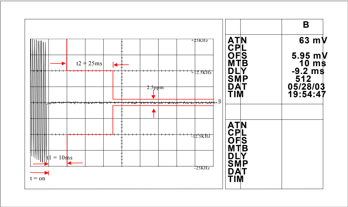
Figure 6I-1: 44 Watts, 12.5 KHz Key-Up Attack Time
