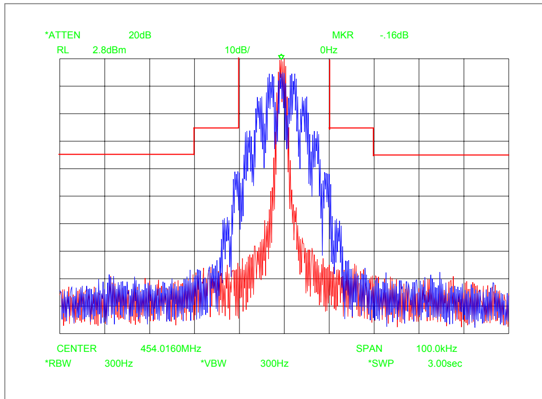
Figure 6E-11: 25 KHz Channel Spacing, 2500 Hz Audio and PL Tone Modulation, Mask B
