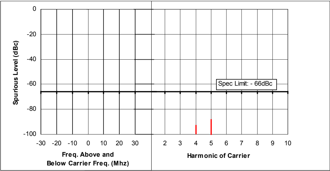
Figure 6F-1: 44 Watts, 438.0125 MHz, 12.5 kHz Channel Spacing
