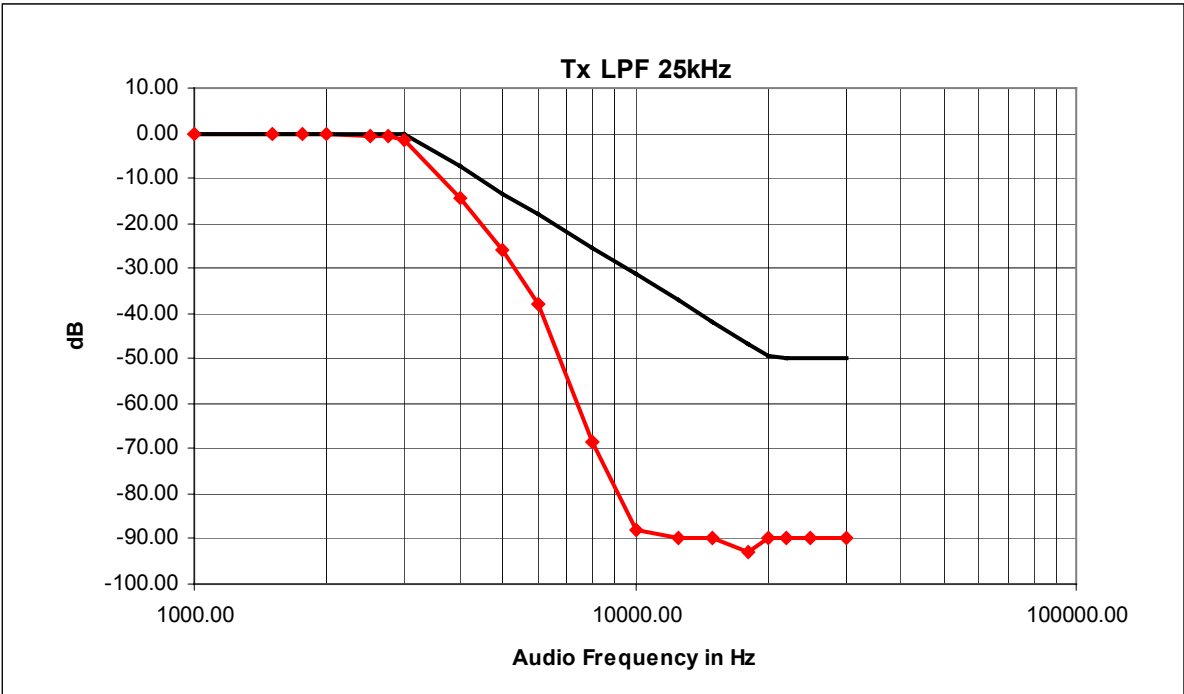
Figure 6C-2: 25 KHz Channel Spacing, Transmit Audio Post Limiter Low Pass Filter Response
