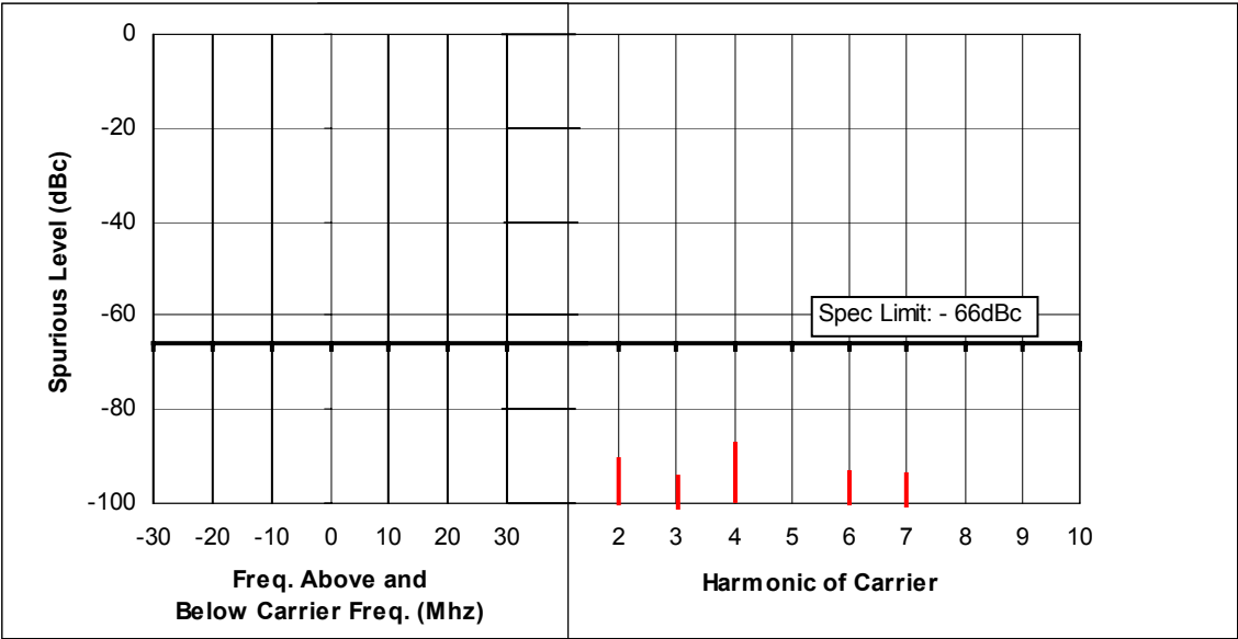
Figure 6F-2: 44 Watts, 454.0125 MHz, 12.5 kHz Channel Spacing
