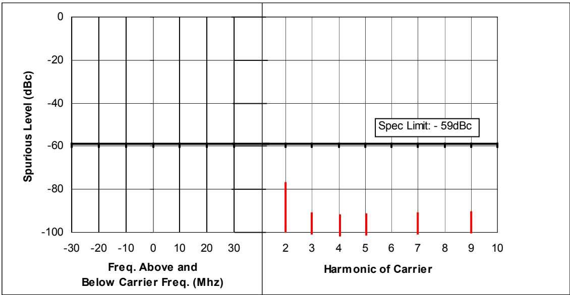
Figure 6F-4: 44 Watts, 438.0125 MHz, 25 kHz Channel Spacing
