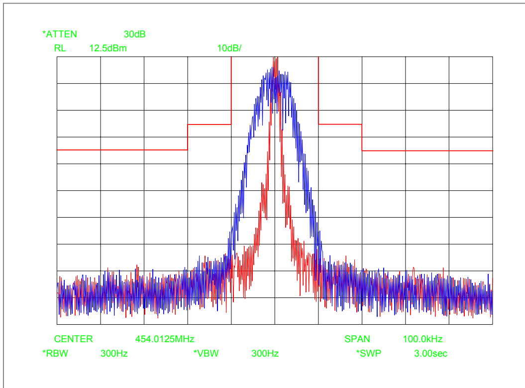
Figure 6E-17: 25 KHz Channel Spacing, DTMF Modulation and PL Tone Modulation, Mask B
