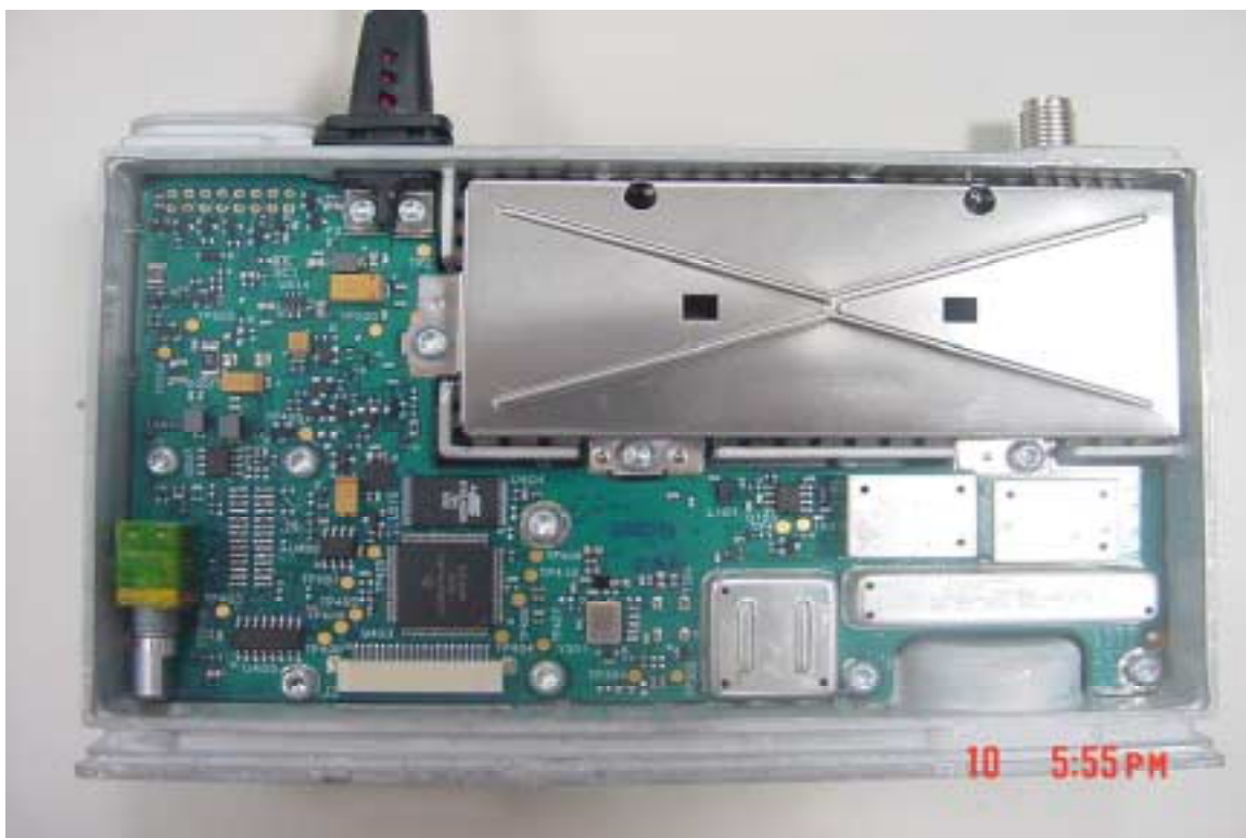
Figure 9-6: Top View of PCB placed in chassis with shield covering transmitter section.
