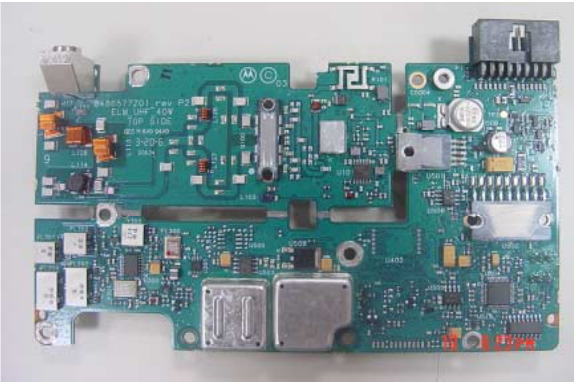
Figure 9-3: Top Side of PCB with shields.
