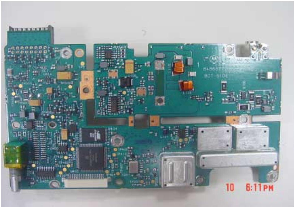
Figure 9-4: Bottom Side of PCB with shields.
