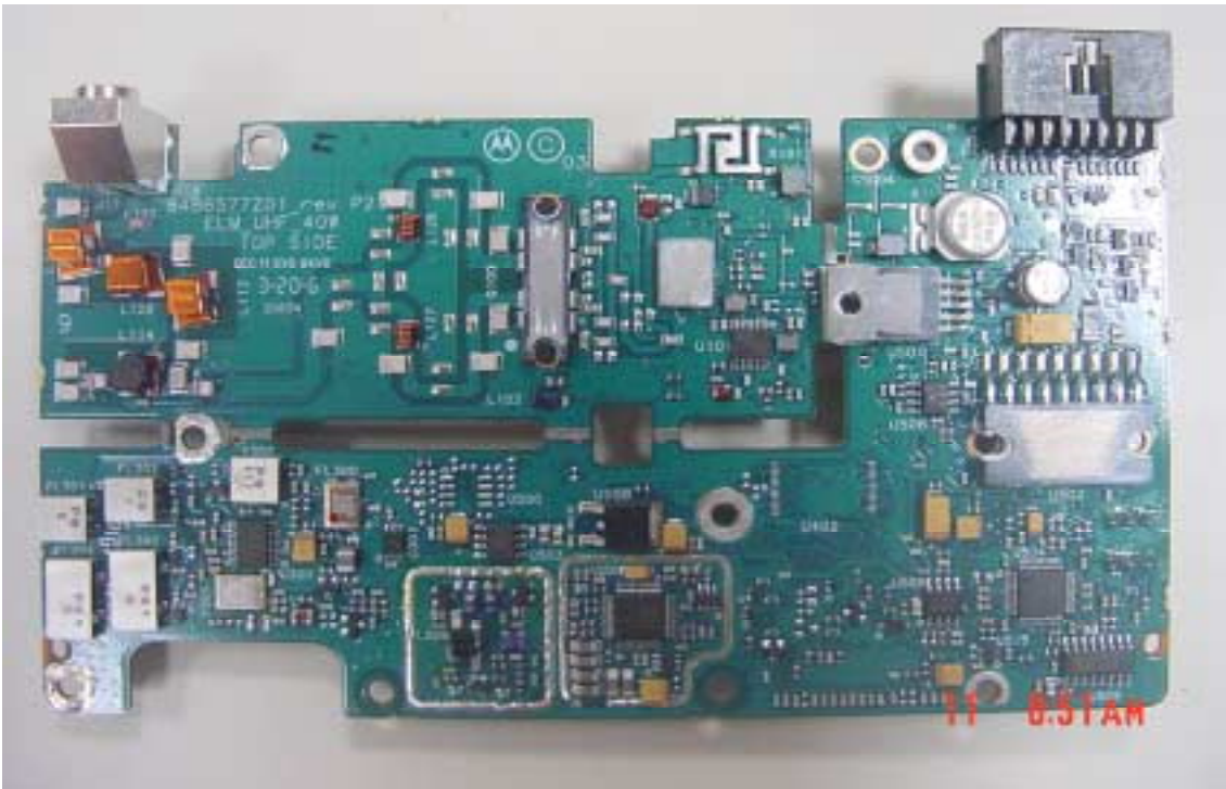
Figure 9-1: Top Side of PCB without shields.
