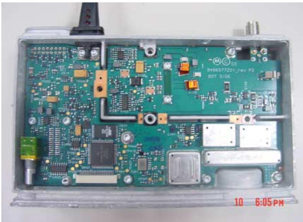
Figure 9-5: Top View of PCB placed in chassis.
