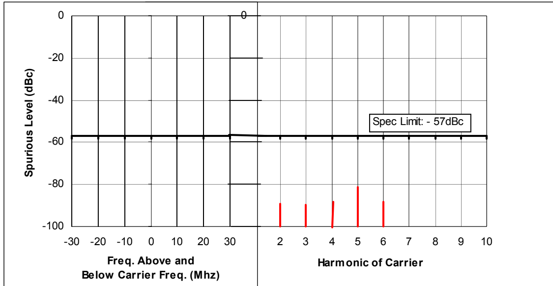
Figure 6F-5: 25 Watts, 421.500 MHz, 25 KHz Channel Spacing
