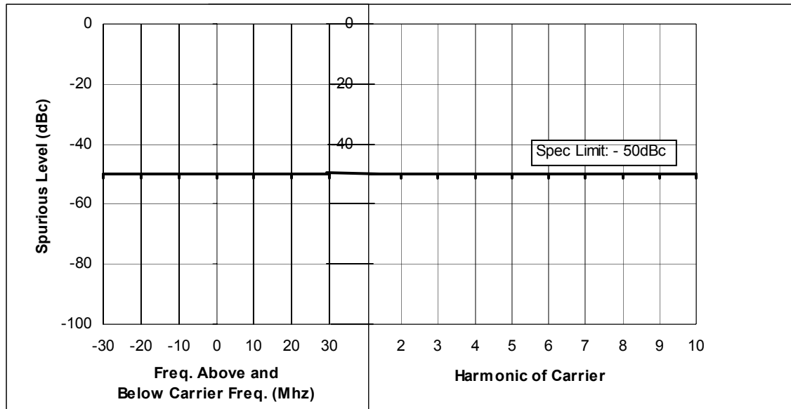
Figure 6F-9: 1 Watts, 439.975 MHz, 12.5 KHz Channel Spacing
