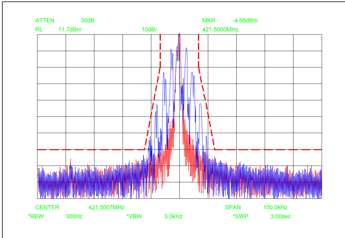
Figure 6E-3: 12.5 KHz Channel Spacing, 2500 Hz Audio and DPL Tone Modulation, Mask D
