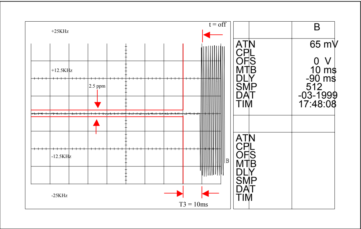
Figure 6I-4: 27 Watts, 25 KHz De-Key Decay Time
