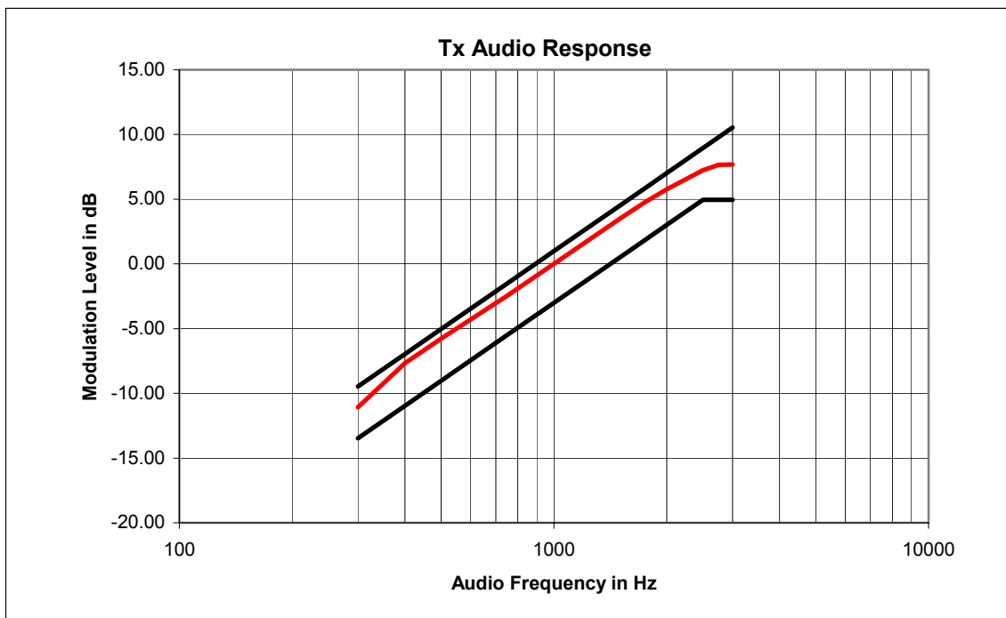
Figure 6B-2: 25 KHz Channel Spacing, Transmit Audio Response
