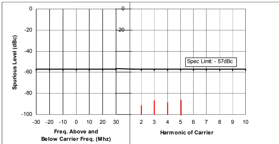
Figure 6F-6: 25 Watts, 439.975 MHz, 25 KHz Channel Spacing
