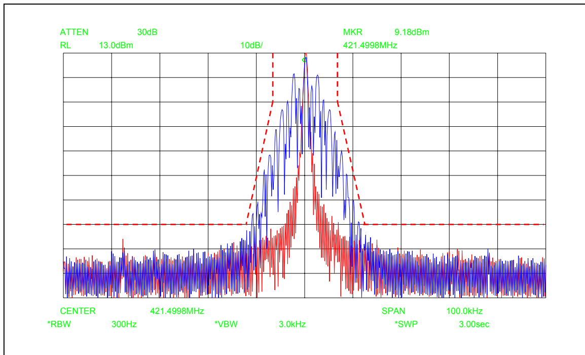
Figure 6E-4: 12.5 KHz Channel Spacing, 2000/3000 Hz FSK Data Modulations Only, Mask D
