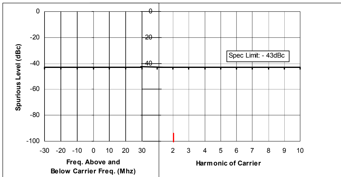
Figure 6F-10: 1 Watts, 403.025 MHz, 25 KHz Channel Spacing
