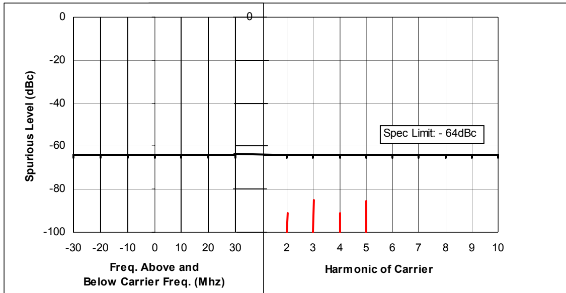
Figure 6F-3: 25 Watts, 439.975 MHz, 12.5 KHz Channel Spacing
