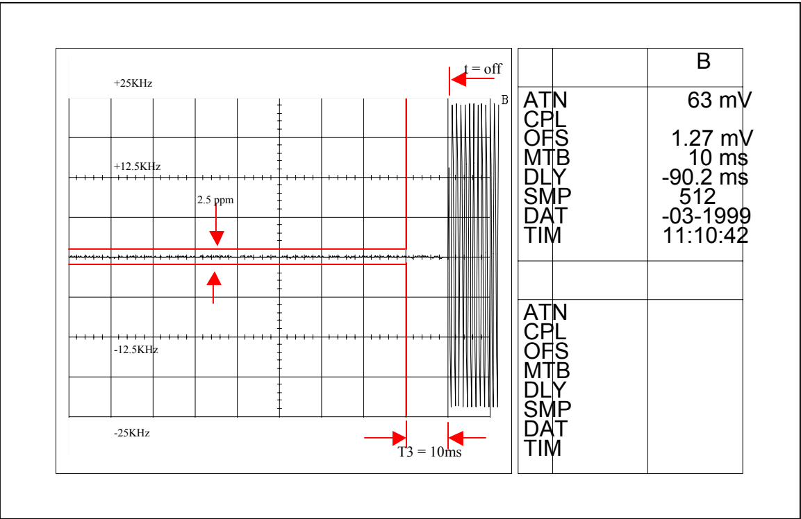
Figure 6I-2: 27 Watts, 12.5 KHz De-Key Decay Time
