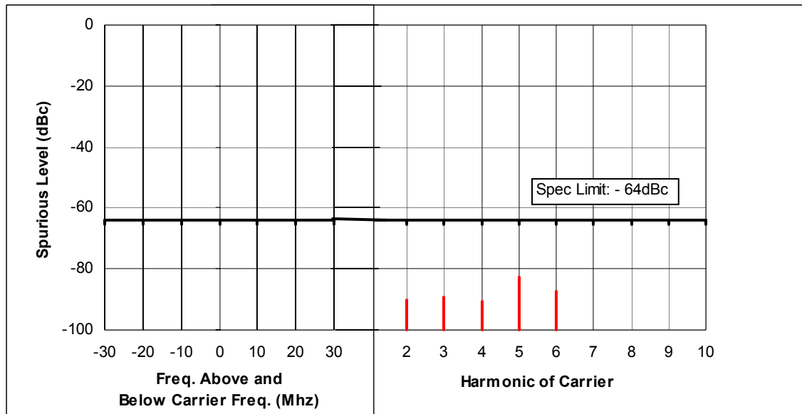
Figure 6F-2: 25 Watts, 421.050 MHz, 12.5 KHz Channel Spacing
