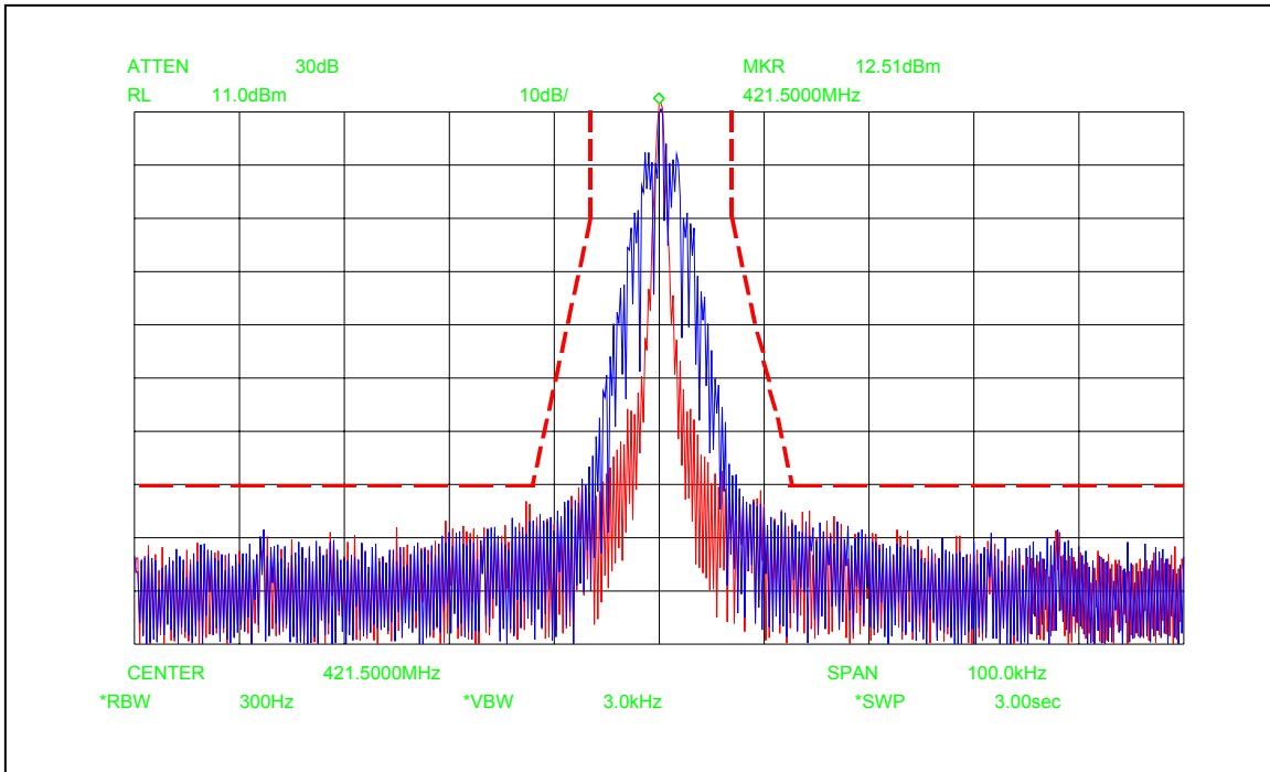
Figure 6E-7: 12.5 KHz Channel Spacing, DTMF Modulation Only, Mask D
