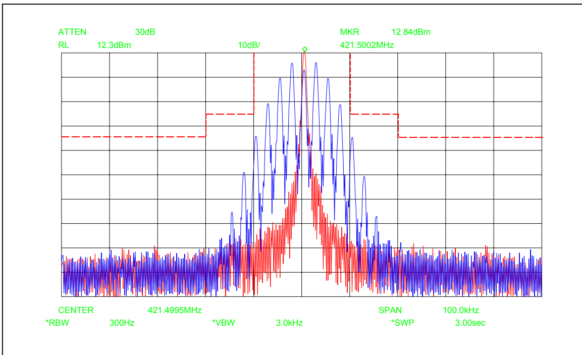
Figure 6E-10: 25 KHz Channel Spacing, 2500 Hz Audio Modulation Only, Mask B
