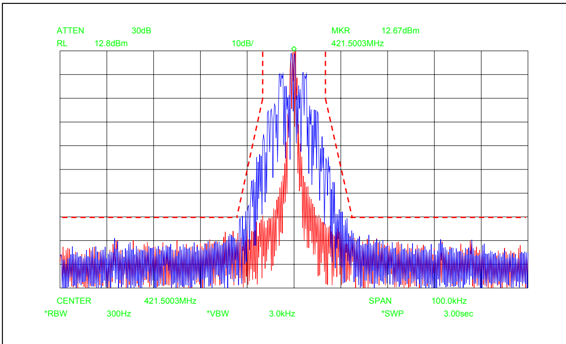
Figure 6E-5: 12.5 KHz Channel Spacing, 2000/3000 Hz FSK Data and PL Tone Modulation, Mask D
