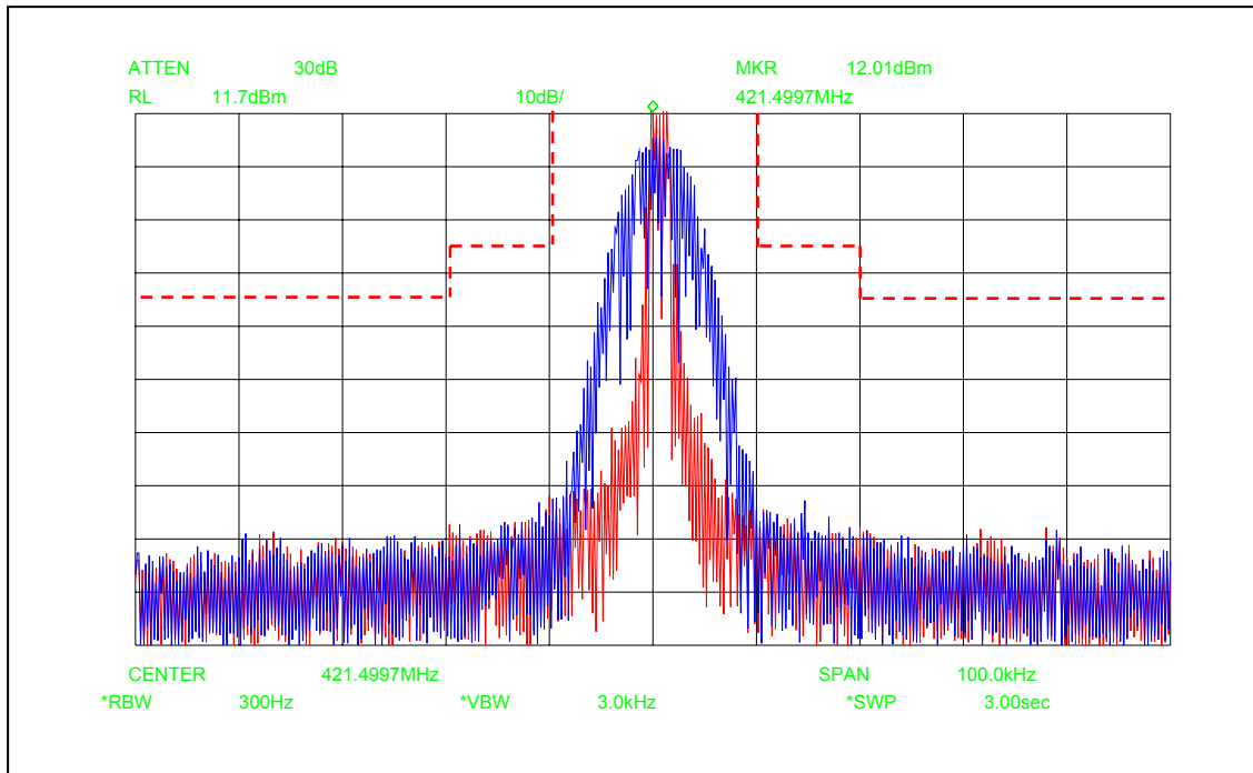
Figure 6E-17: 25 KHz Channel Spacing, DTMF Modulation and PL Tone Modulation, Mask B
