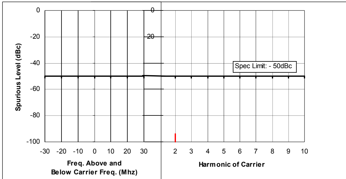
Figure 6F-7: 1 Watts, 403.025 MHz, 12.5 KHz Channel Spacing
