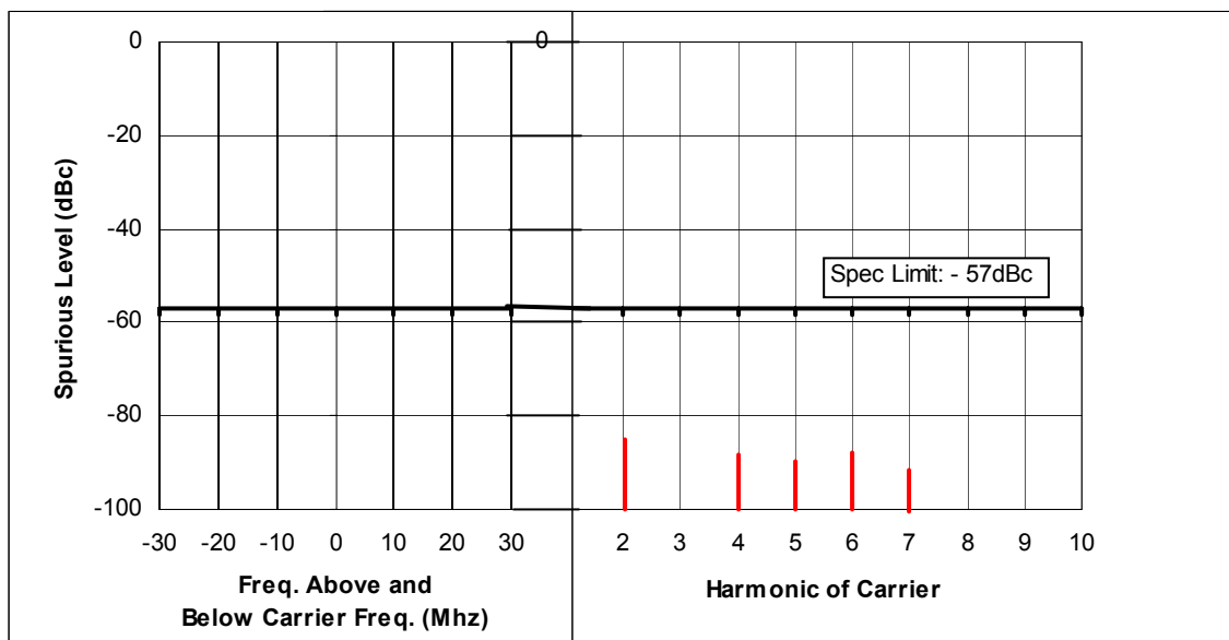
Figure 6F-4: 25 Watts, 403.025 MHz, 25 KHz Channel Spacing
