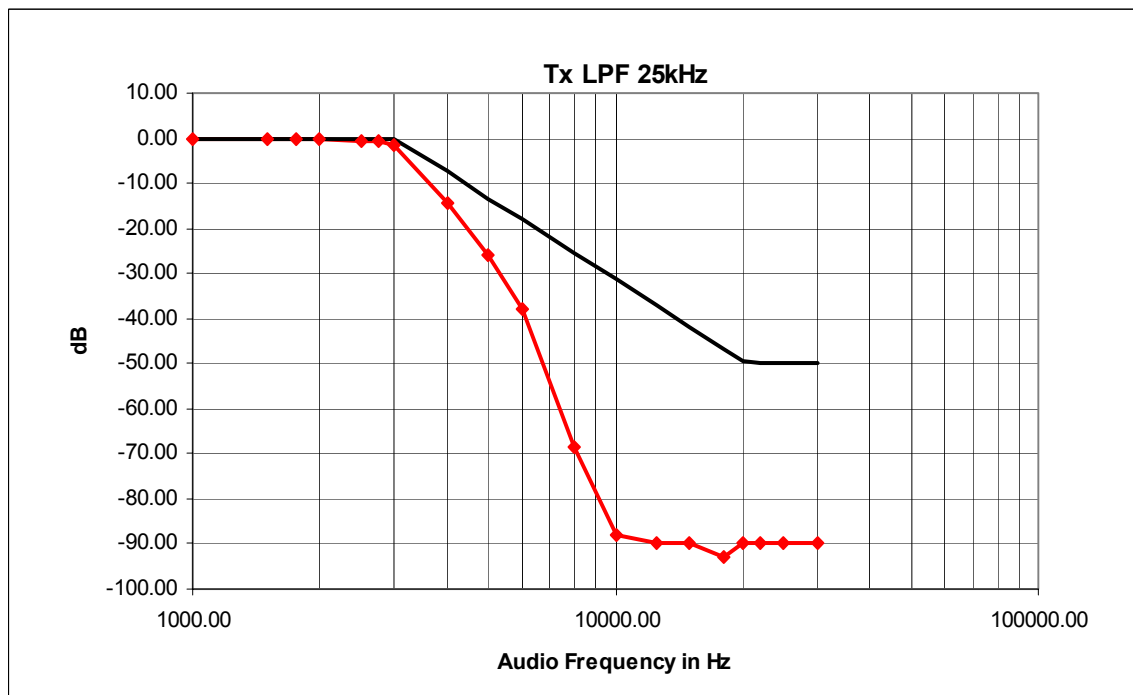
Figure 6C-2: 25 KHz Channel Spacing, Transmit Audio Post Limiter Lowpass Filter Response
