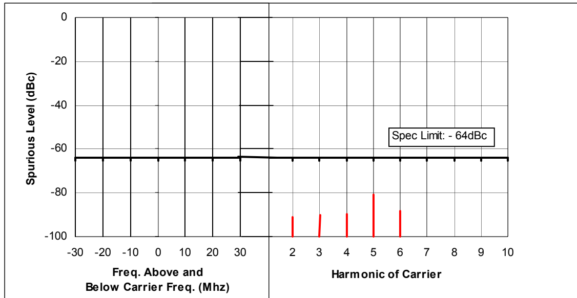
Figure 6F-1: 25 Watts, 403.025 MHz, 12.5 KHz Channel Spacing
