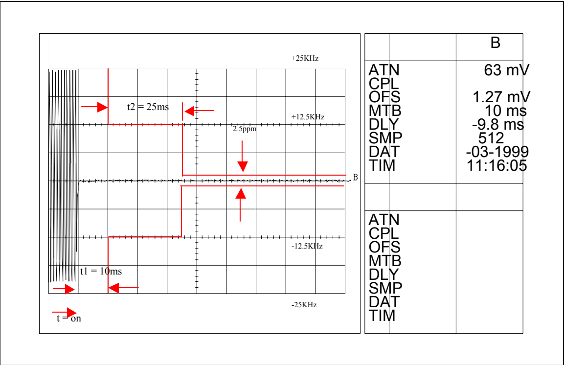
Figure 6I-1: 27 Watts, 12.5 KHz Key-Up Attack Time
