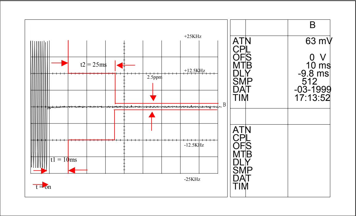
Figure 6I-7: 1 Watts, 25 KHz Key-Up Attack Time
