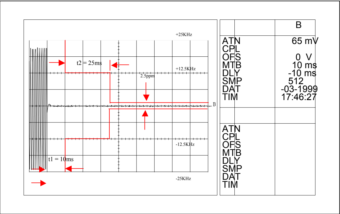
Figure 6I-3: 27 Watts, 25 KHz Key-Up Attack Time
