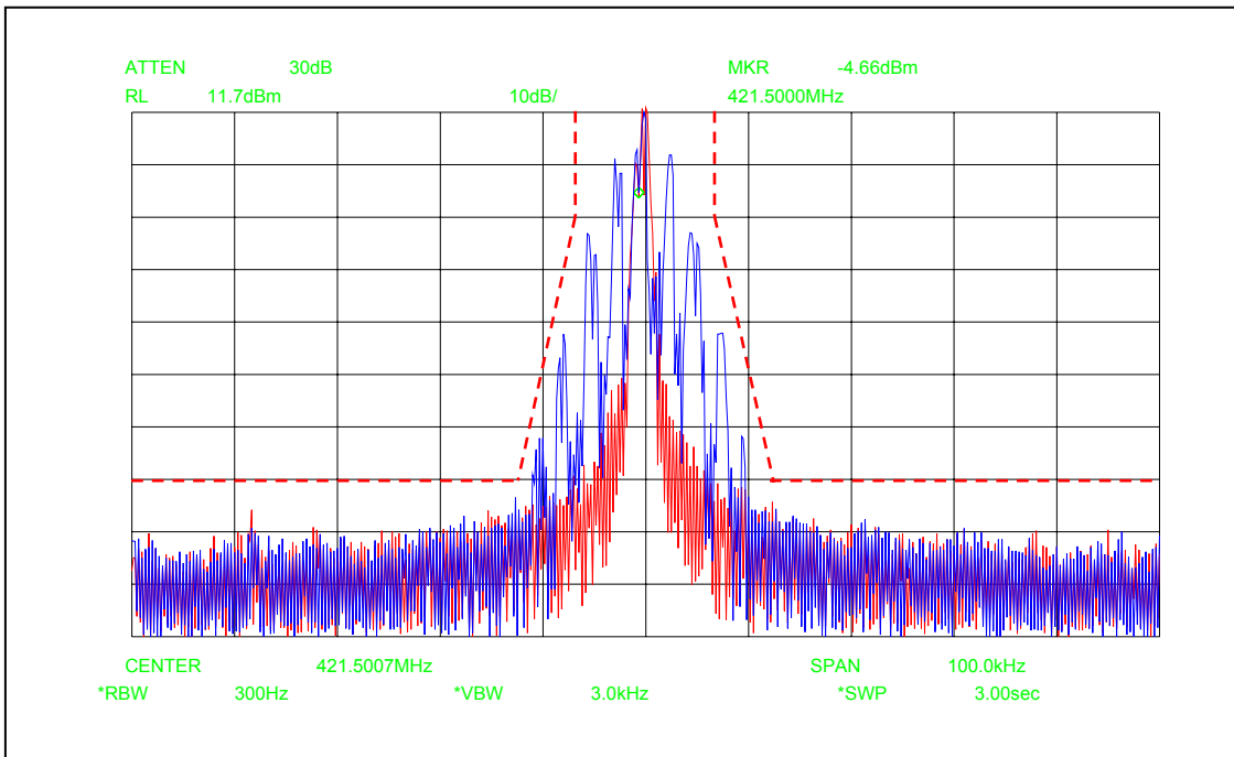
Figure 6E-2: 12.5 KHz Channel Spacing, 2500 Hz Audio and PL Tone Modulation, Mask D
