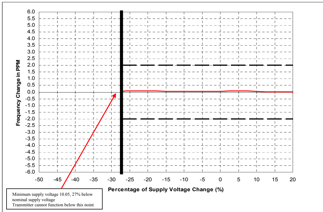
Figure 6H-2: Frequency Stability vs. Supply Voltage
