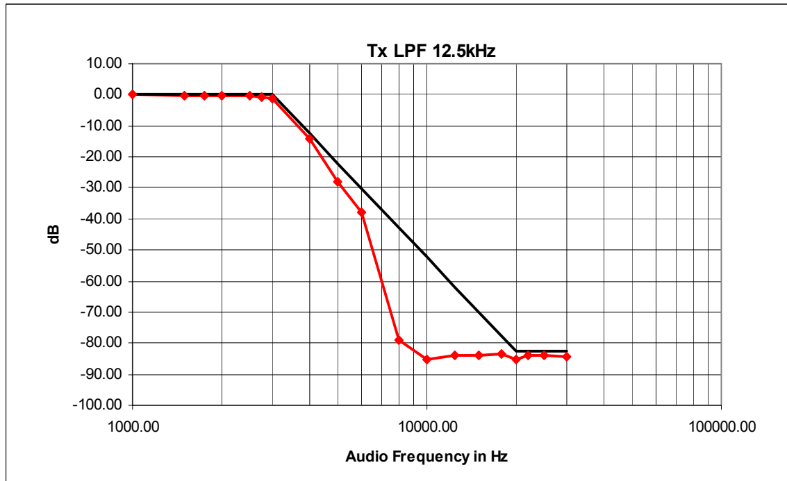
Figure 6C-1: 12.5 KHz Channel Spacing, Transmit Audio Post Limiter Lowpass Filter Response
