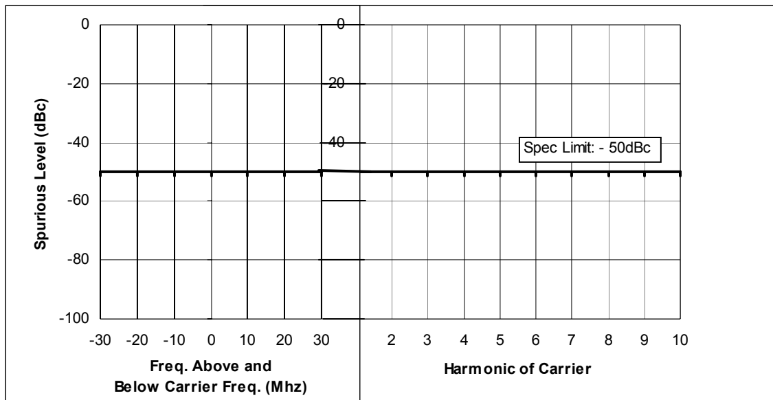
Figure 6F-8: 1 Watts, 421.500 MHz, 12.5 KHz Channel Spacing
