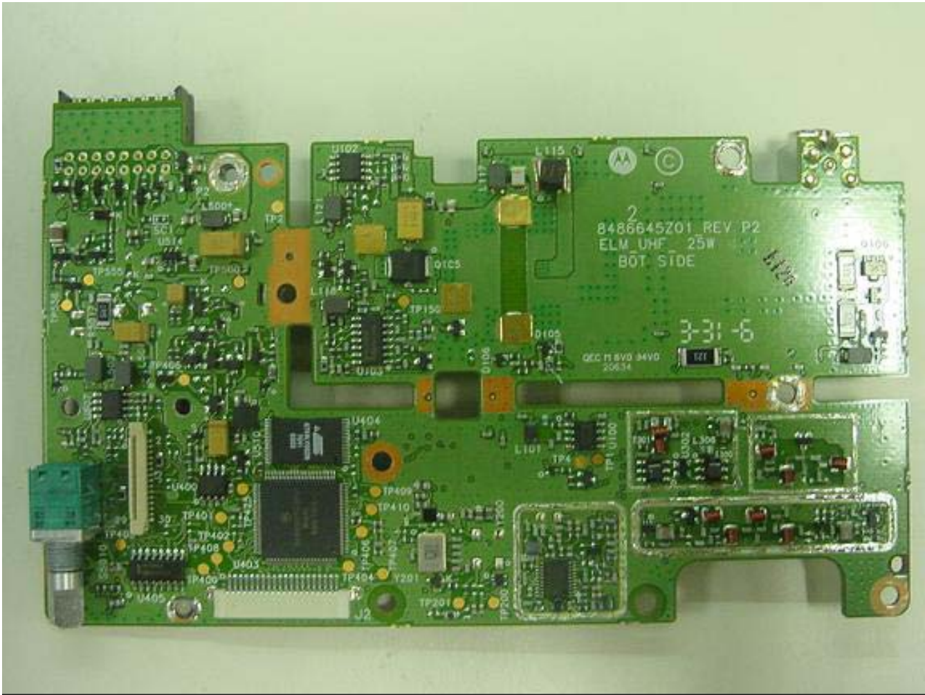
Figure 9-2: Bottom Side of PCB without shields.
