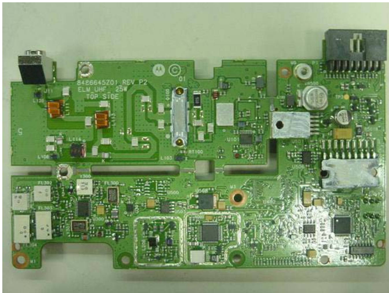
Figure 9-1: Top Side of PCB without shields.
