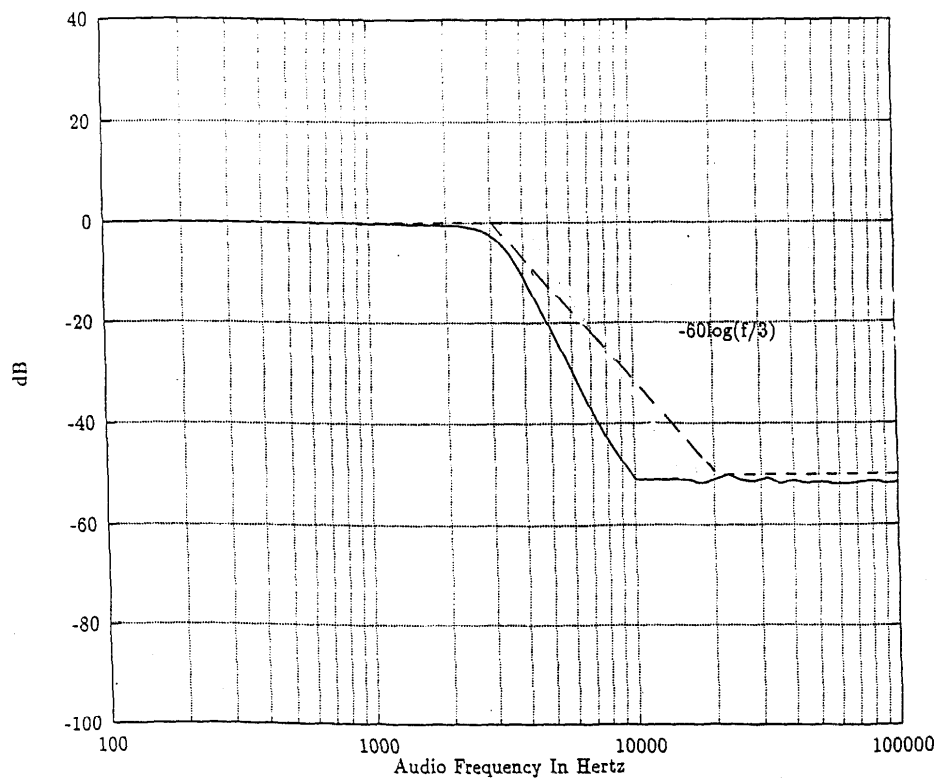
Transmit Audio Post Limiter Lowpass Filter Response - 25 kHz Channel Spacing
