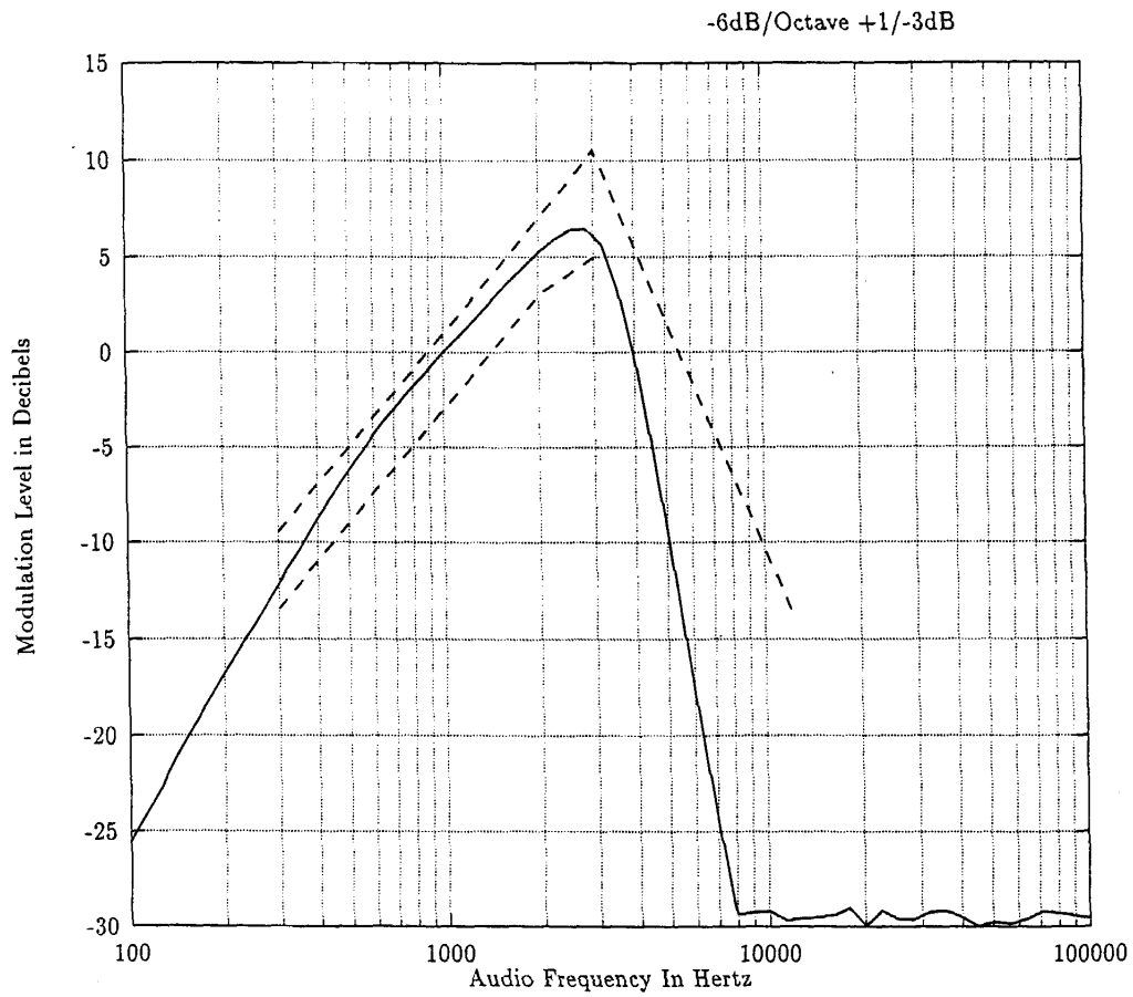
Transmit Audio Response - 25 kHz Channel Spacing
