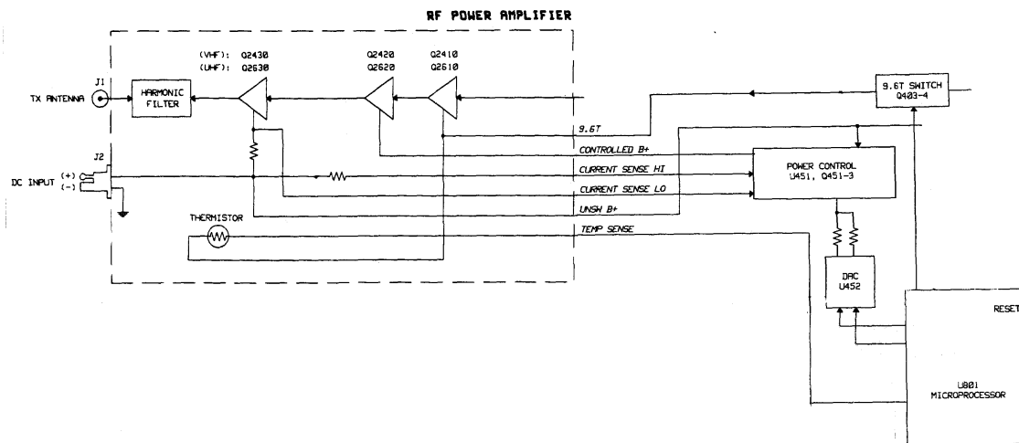
Figure 4.4 - Transmitter Power Limiting Block Diagram
