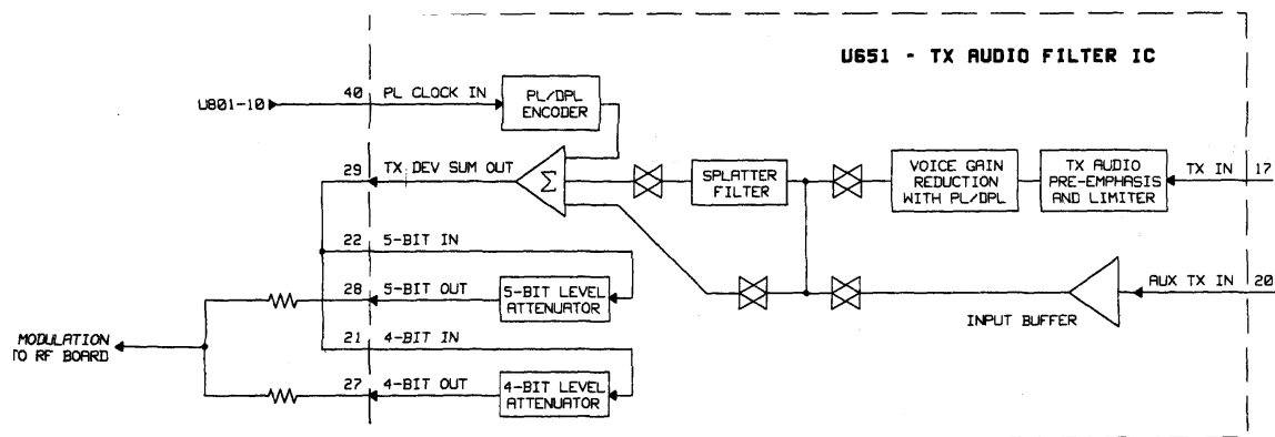
Figure 4.2 – Transmitter Modulation Limiting and Lowpass Filtering
