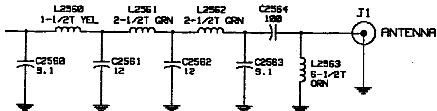
Figure 4.3 – Transmitter Lowpass Filter
