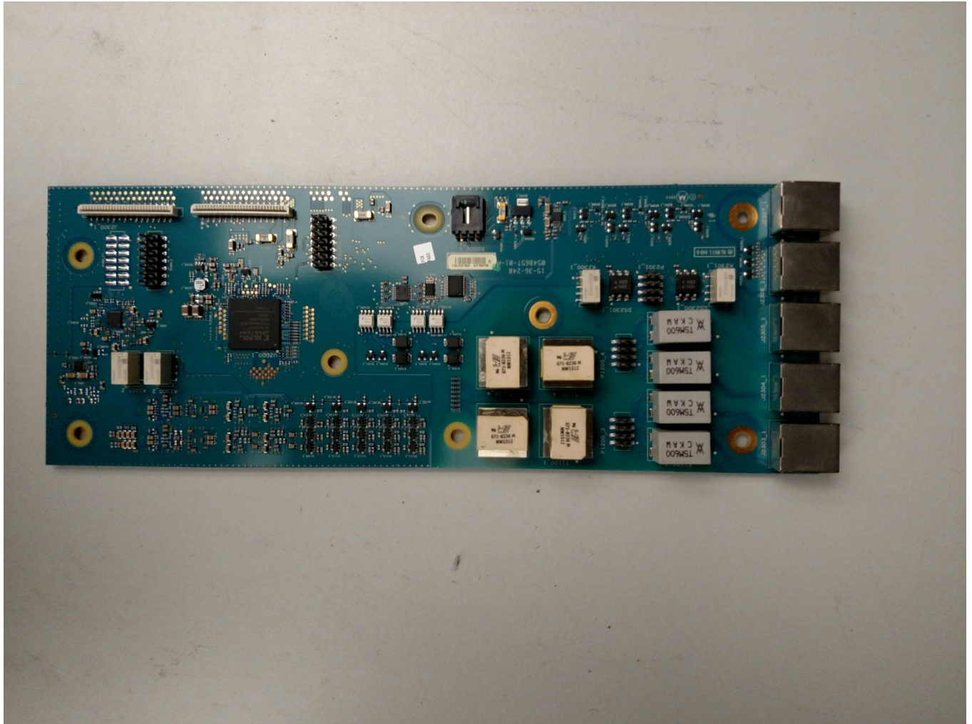
Internal Front View – Wireline Board Top View
