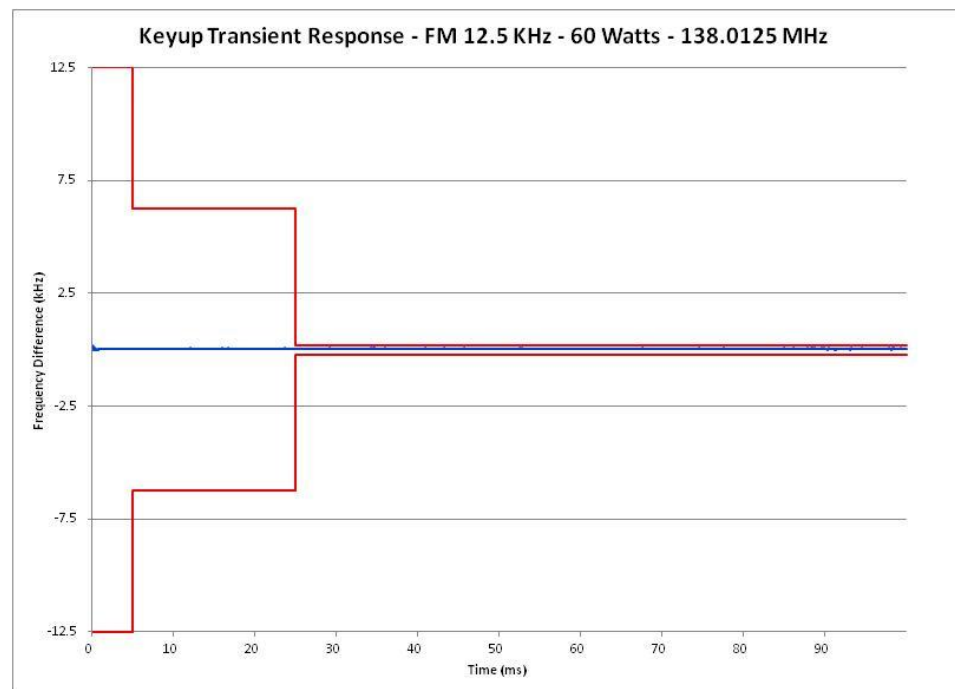
E1-9.7 Frequency Transient Behavior, 12.5 kHz Channel Key-Up, 138.0125 MHz
