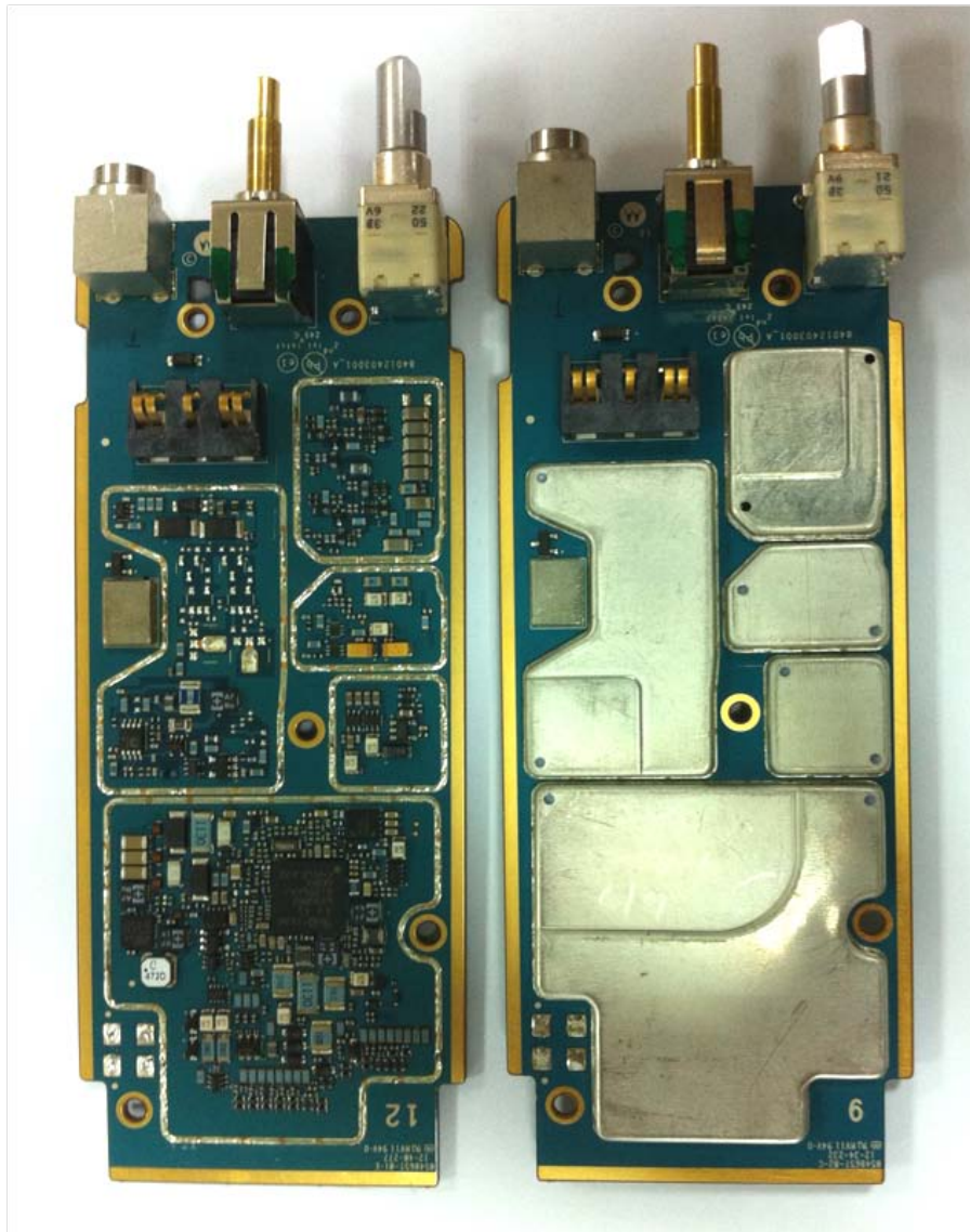
RF board without & with Shields (Bottom)
