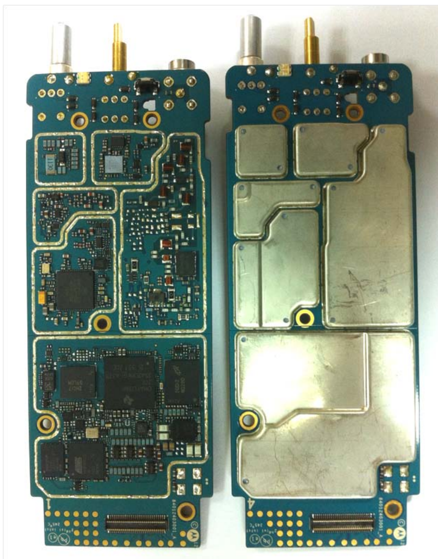
RF board without & with Shields (Top)
