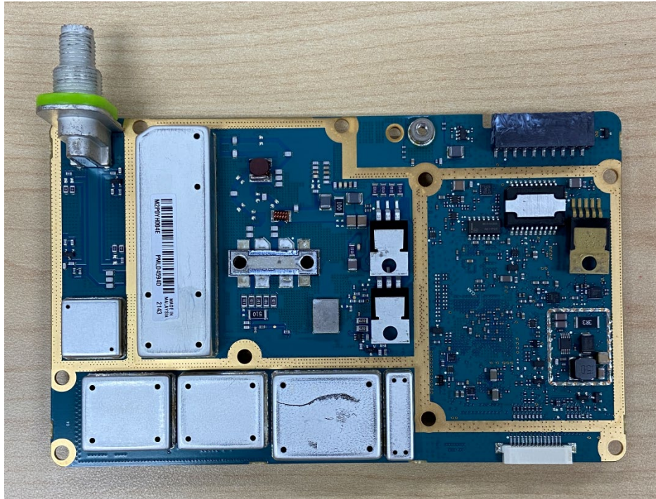
Exhibit 9A - RF board with Shields (Top)
