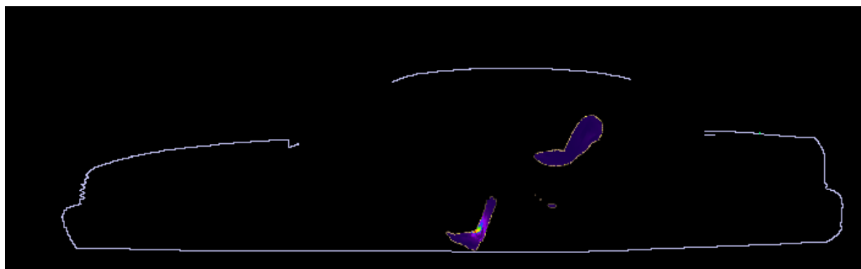
Figure 3. SAR distribution at 140.0125 MHz in the passenger model located in the center of the back seat, produced by the trunk-mount HAD4006A antenna. The contour plot is relative to the plane where the peak 1-g average SAR for this exposure condition occurs.
