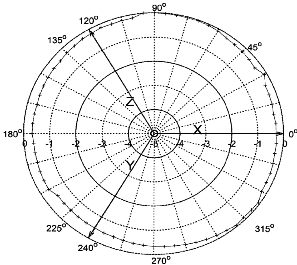
Figure 1: Probe Isotropic Response Chart.
