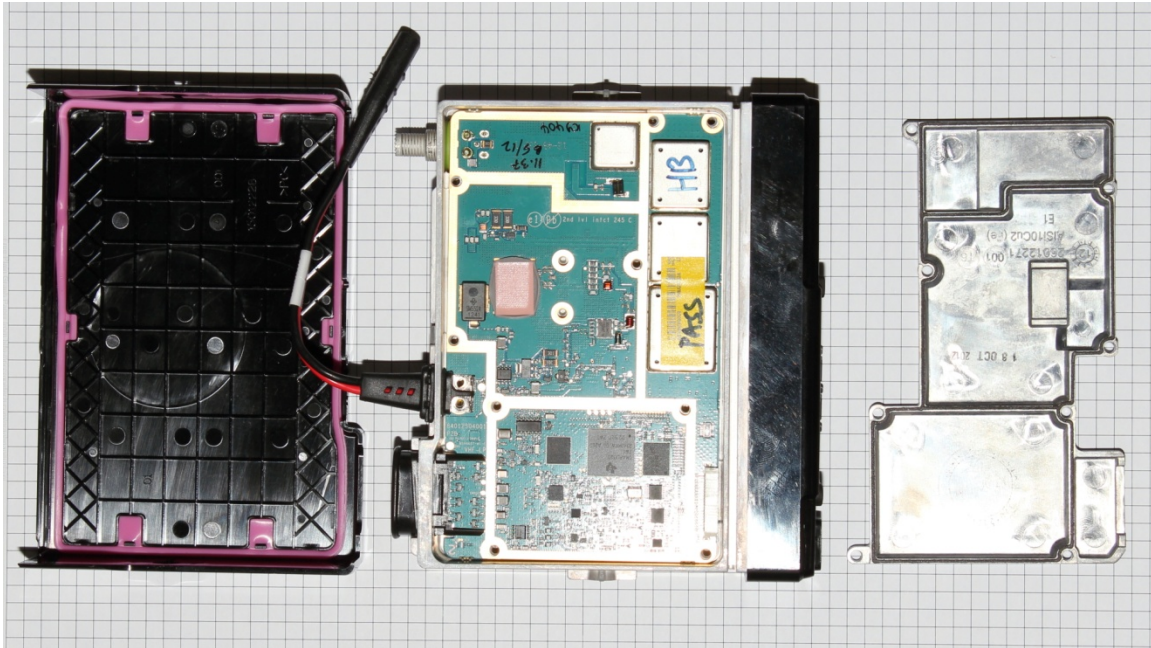
TOP VIEW WITH DECORATIVE COVER AND CHASSIS TOP COVER REMOVED (MATING SURFACES OF TOP COVER AND CIRCUIT BOARD IN CHASSIS ARE SHOWN)
