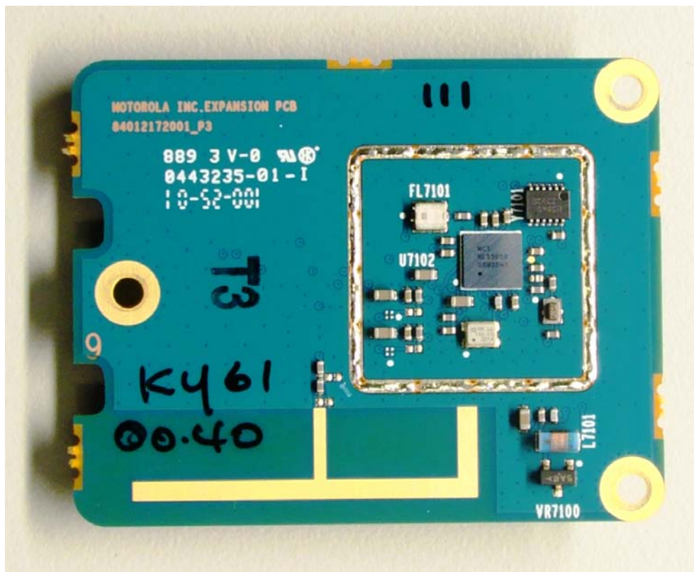
FRONT VIEW OF BLUETOOTH/GPS BOARD WITH SHIELD REMOVED
