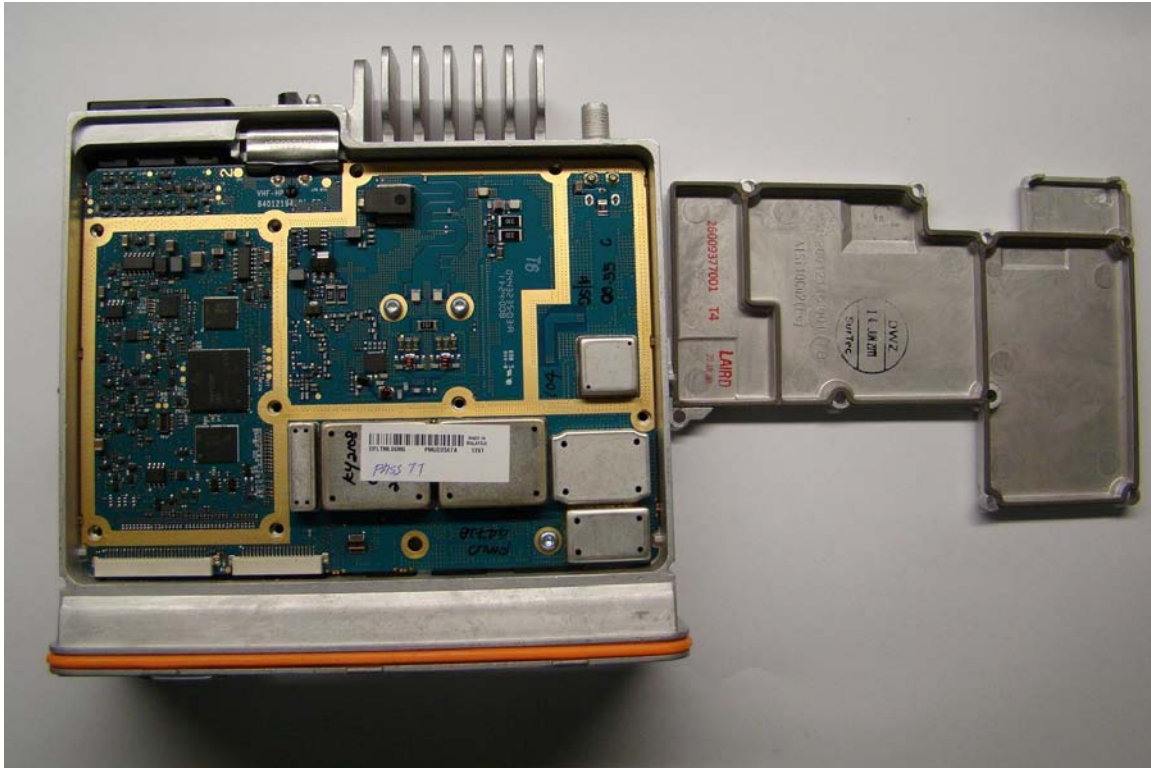
TOP VIEW WITH CHASSIS TOP COVER REMOVED (MATING SURFACES OF TOP COVER AND CIRCUIT BOARD IN CHASSIS ARE SHOWN)
