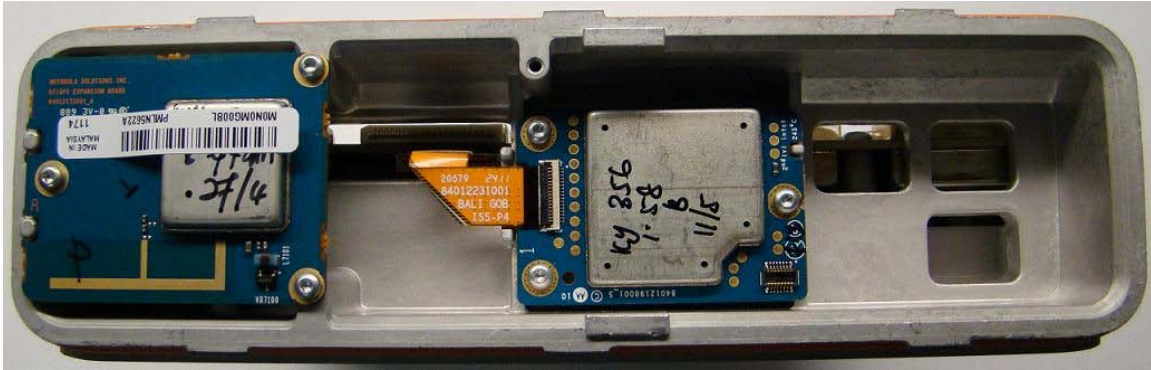
FRONT VIEW WITH BLUETOOTH/GPS BOARD INSTALLED ON THE LEFT AND GENERIC OPTION BOARD INSTALLED ON THE RIGHT
