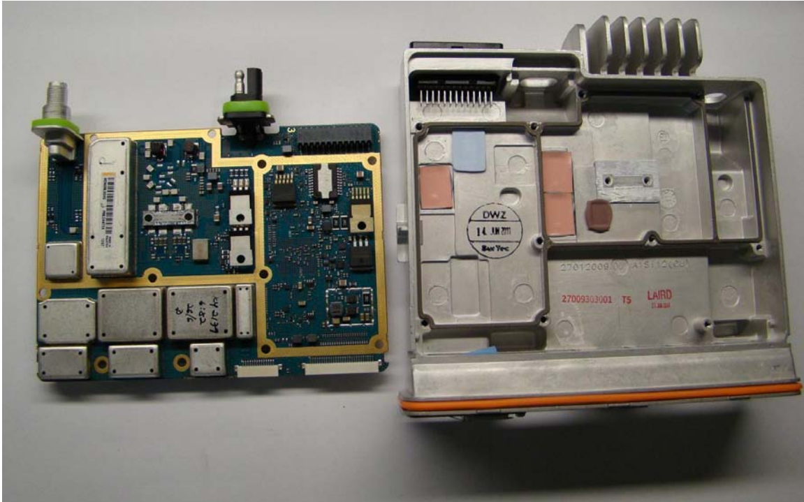
TOP VIEW WITH CIRCUIT BOARD REMOVED FROM CHASSIS (MATING SURFACES OF CIRCUIT BOARD AND CHASSIS ARE SHOWN)
