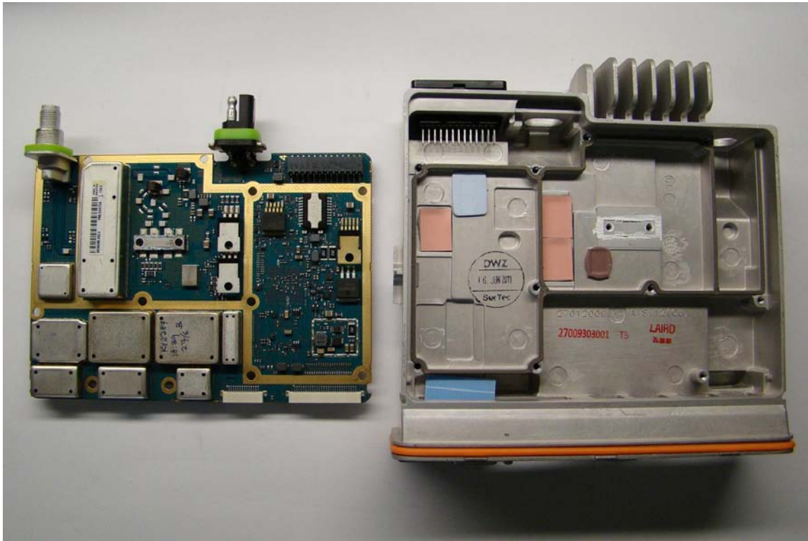
TOP VIEW WITH CIRCUIT BOARD REMOVED FROM CHASSIS (MATING SURFACES OF CIRCUIT BOARD AND CHASSIS ARE SHOWN)
