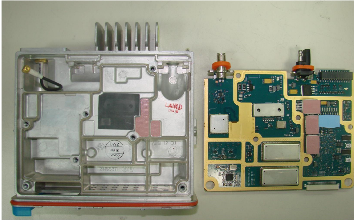
TOP VIEW OF GPS MODEL WITH CIRCUIT BOARD REMOVED FROM CHASSIS (MATING SURFACES OF CIRCUIT BOARD AND CHASSIS ARE SHOWN)
