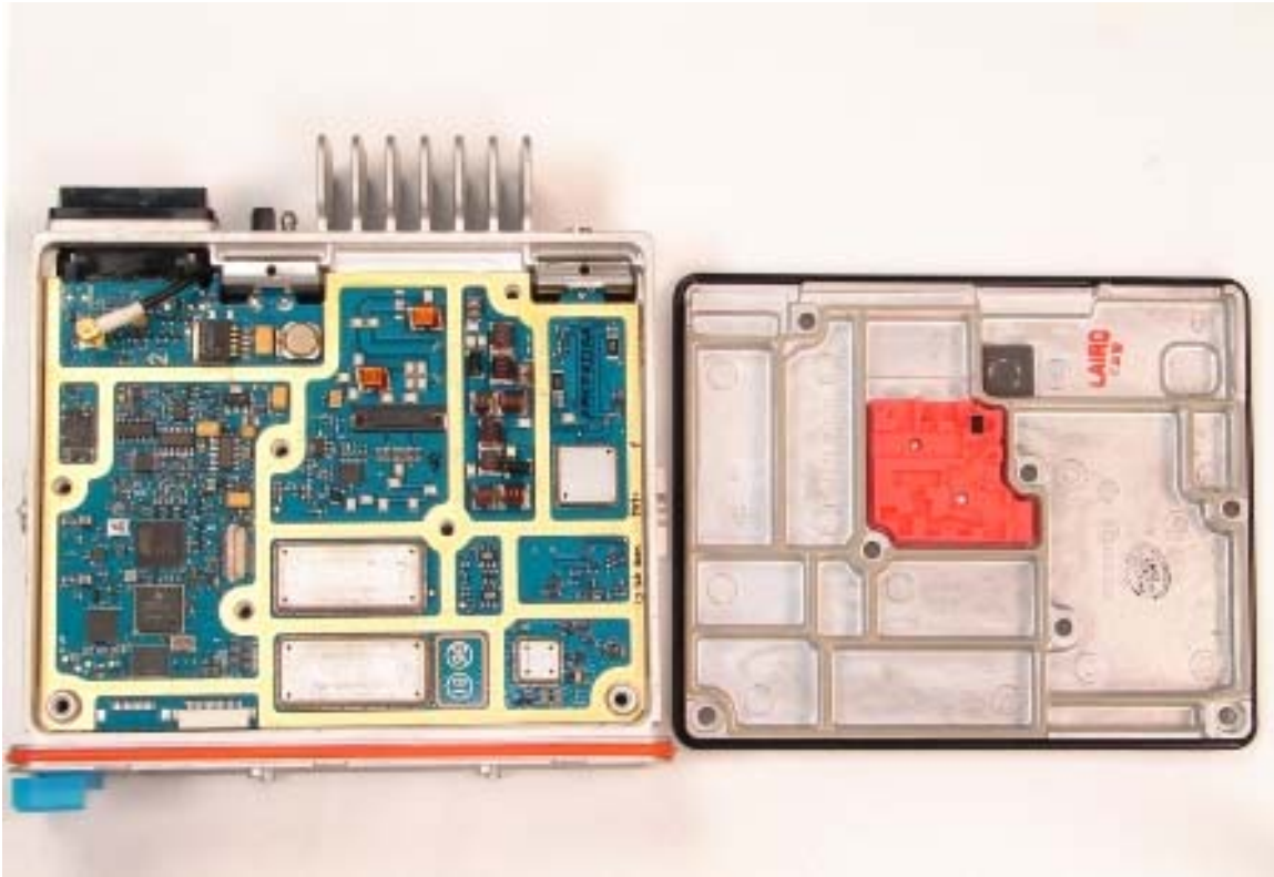
TOP VIEW OF GPS MODEL WITH CHASSIS TOP COVER REMOVED (MATING SURFACES OF TOP COVER AND CIRCUIT BOARD IN CHASSIS ARE SHOWN)
