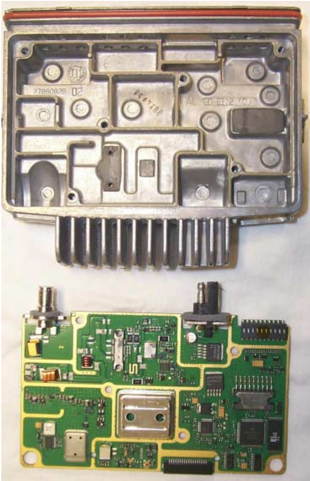
TOP VIEW WITH CIRCUIT BOARD REMOVED FROM CHASSIS (MATING SURFACES OF CIRCUIT BOARD AND CHASSIS ARE SHOWN)
