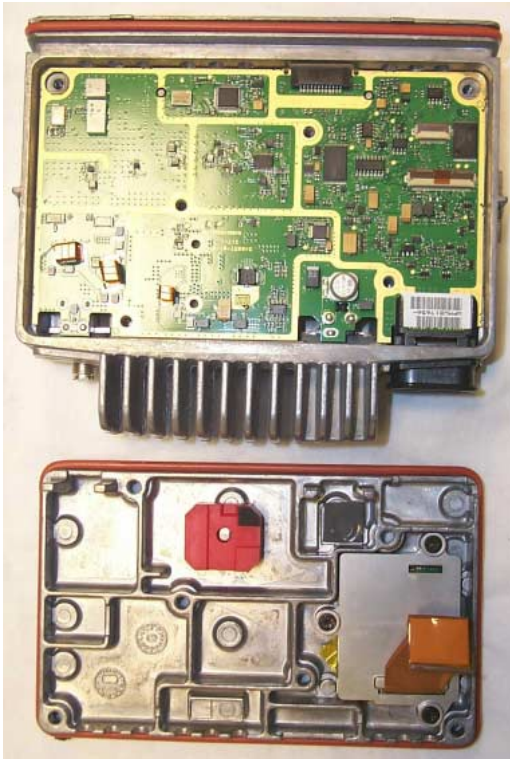
TOP VIEW WITH CHASSIS TOP COVER REMOVED (MATING SURFACES OF TOP COVER AND CIRCUIT BOARD ARE SHOWN)
