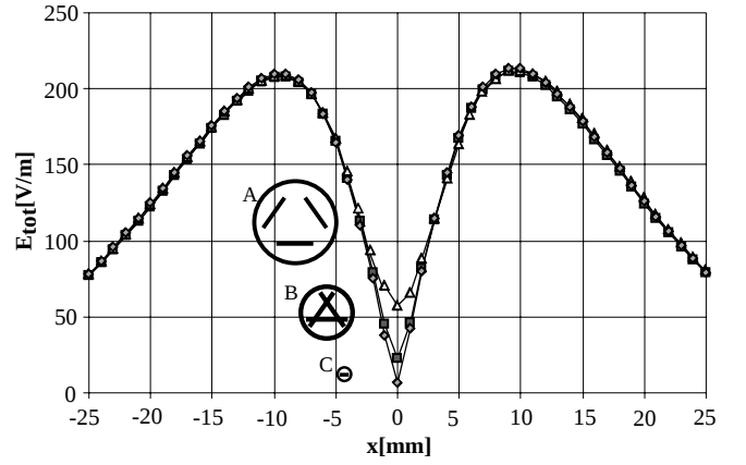
Fig. 16. Total E-field along the x-axis at d=5 mm measured with probe A ( \Delta ), probe B ( \square ) and probe C ( \diamond ). Measurement setup according to Fig.15.
