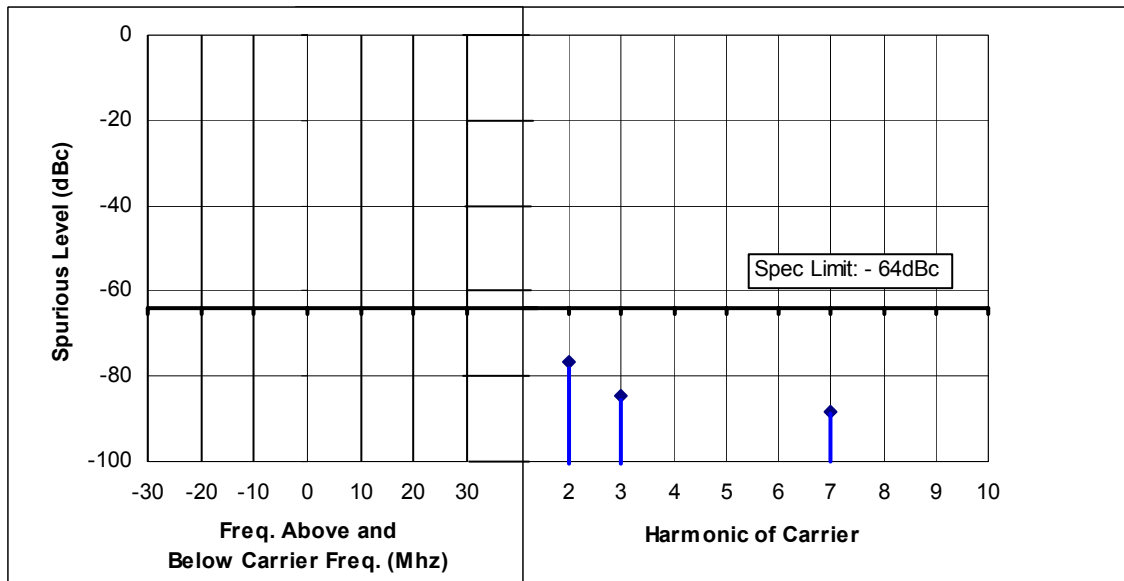
Figure 6F-8: 25 Watts, 149.00 MHz, 12.5 kHz Channel Spacing
