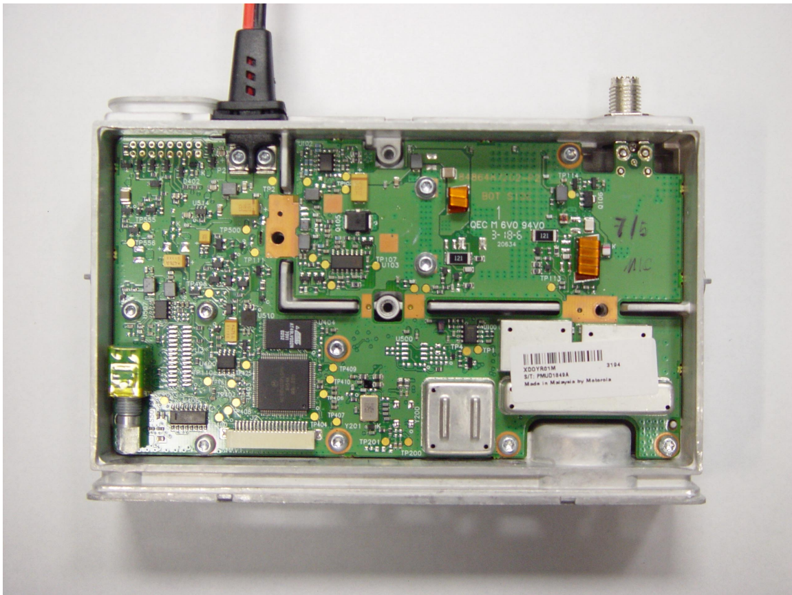
TOP VIEW OF RADIO WITH PA SHIELD REMOVED
