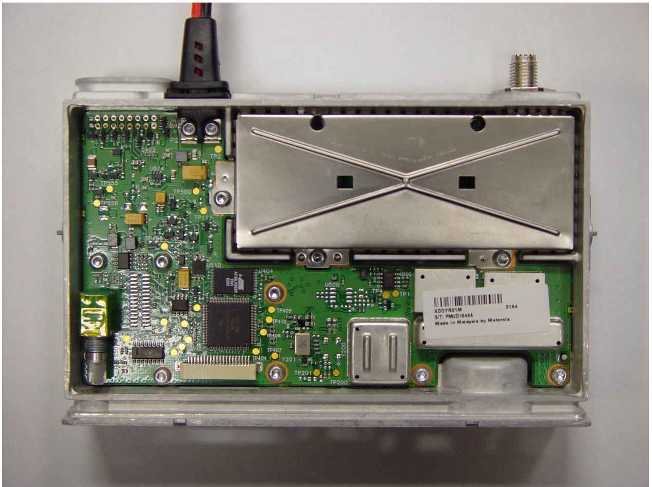
TOP VIEW OF RADIO WITH CHASSIS SHIELD REMOVED
