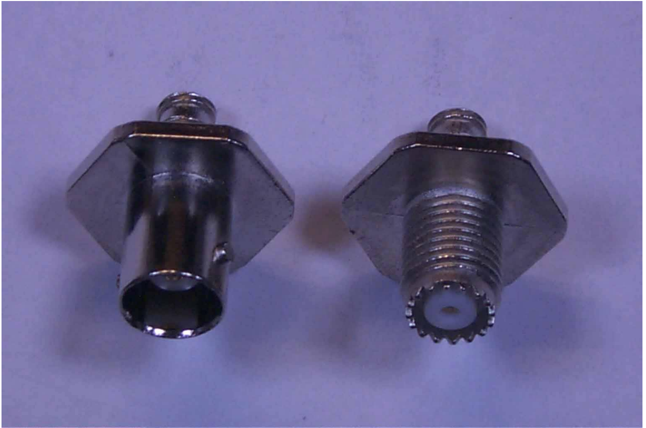
CLOSE-UP VIEWS OF BNC (LEFT) AND MINI-UHF (RIGHT) ANTENNA CONNECTORS
