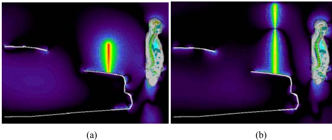
Figure 1: Bystander models using (a) a quarter wave antenna operating at 146 MHz and (b) a 3 dBi gain antenna operating at 155 MHz. A time snapshot of the E-field is displayed in both cases.
