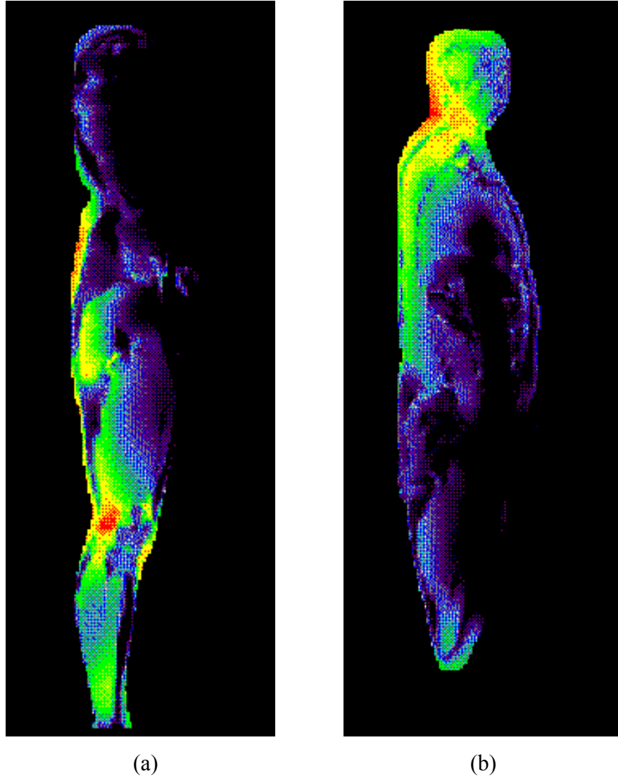
Figure 3: SAR distribution in bystander models produced by (a) a quarter wave antenna operating at 146 MHz (sagittal plane through the leg), and (b) a 3 dBi gain antenna operating at 155 MHz (mid sagittal plane), mounted on the trunk of the vehicle at 60 cm from the body.
