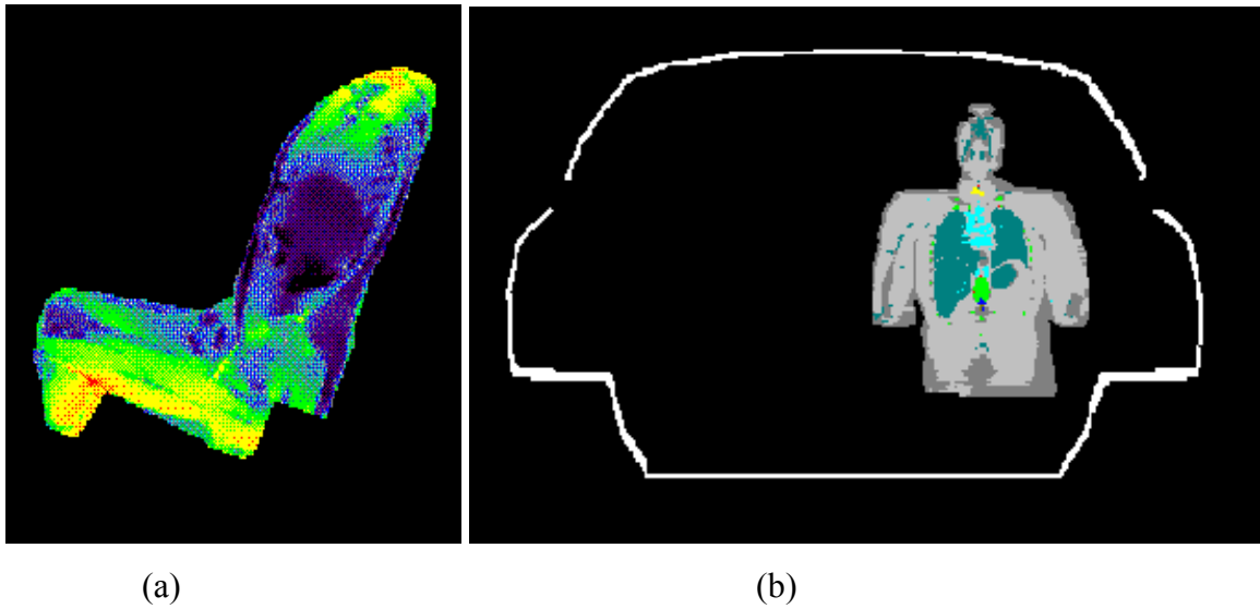
Figure 5: SAR distribution in the passenger model through the plane where the peak SAR occurs (a) placed laterally in the back seat (b), with a trunk-mount antenna operating at 174 MHz.
