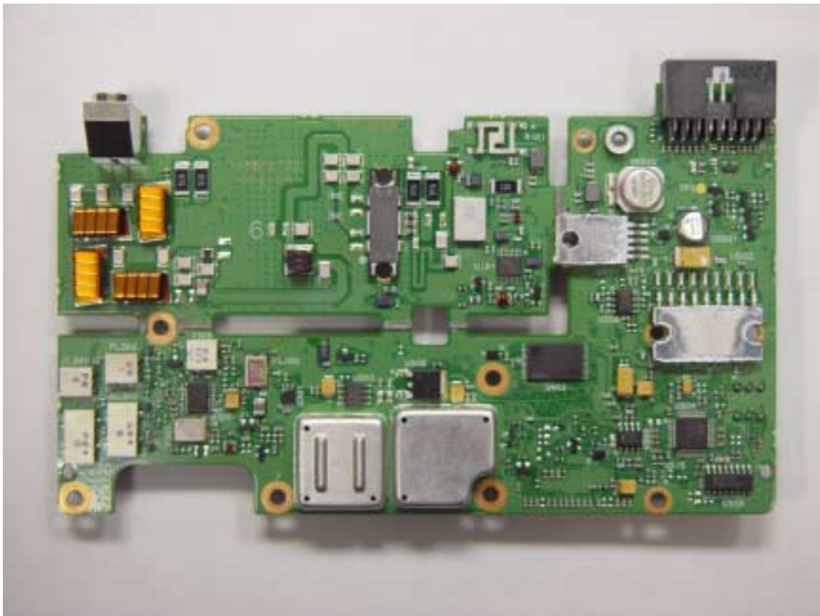
BOTTOM VIEW OF CIRCUIT BOARD REMOVED FROM CHASSIS
