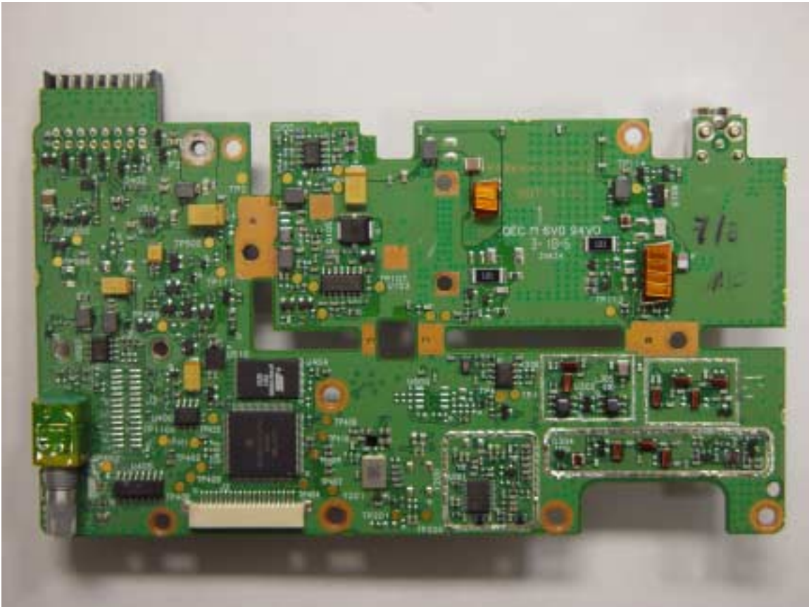
TOP VIEW OF CIRCUIT BOARD WITH ALL SHIELDS REMOVED
