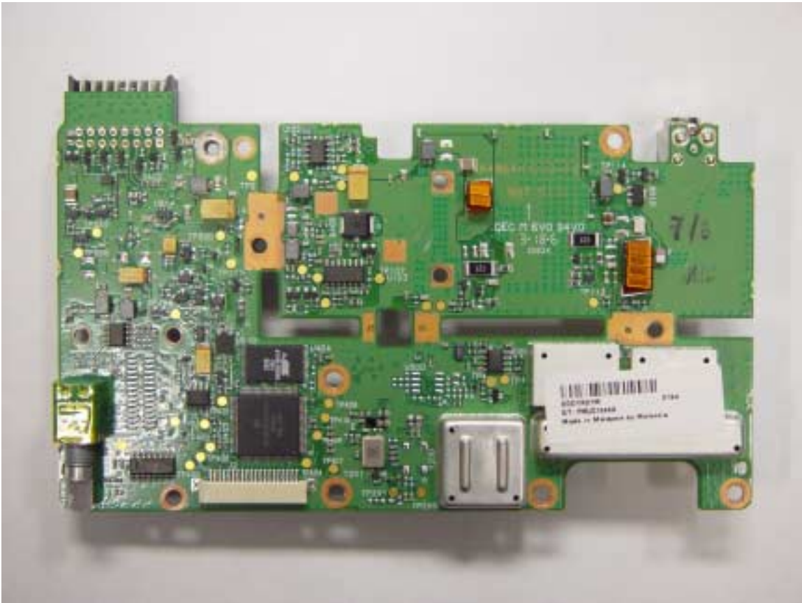
TOP VIEW OF CIRCUIT BOARD REMOVED FROM CHASSIS
