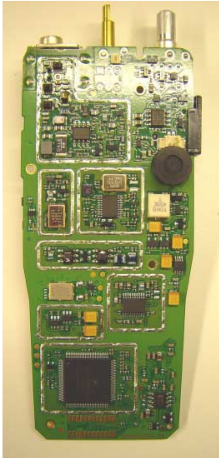
VIEW OF HOUSING-SIDE OF CIRCUIT BOARD WITH ALL SHIELDS REMOVED
