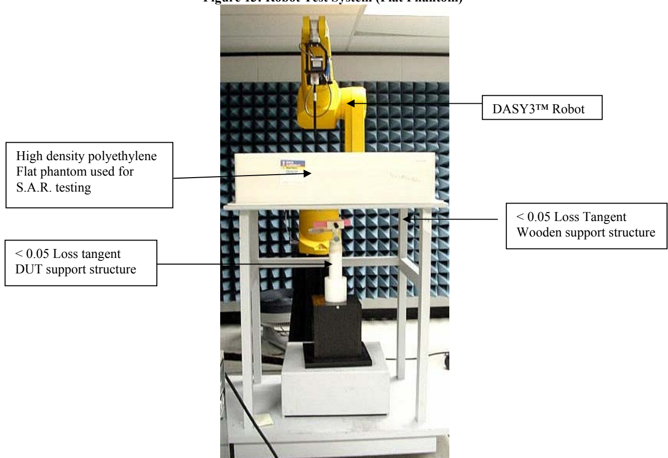
Figure 13: Robot Test System (Flat Phantom)
