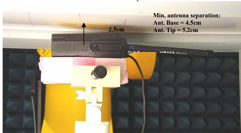
Figure 10. Assessment at the Body w/ back towards phantom and antenna @ 2.5cm With attached audio accessory model HMN9030A
