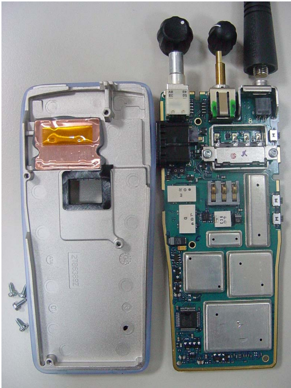
VIEW OF CIRCUIT BOARD REMOVED FROM CHASSIS (MATING SURFACES OF CIRCUIT BOARD AND CHASSIS ARE SHOWN)
