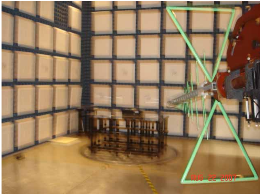
Test Set-up for Radiated Emissions, 30MHz to 1GHz - Vertical
