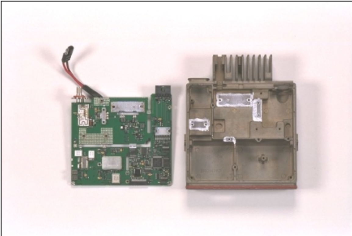
(PC board bottom side shown)
