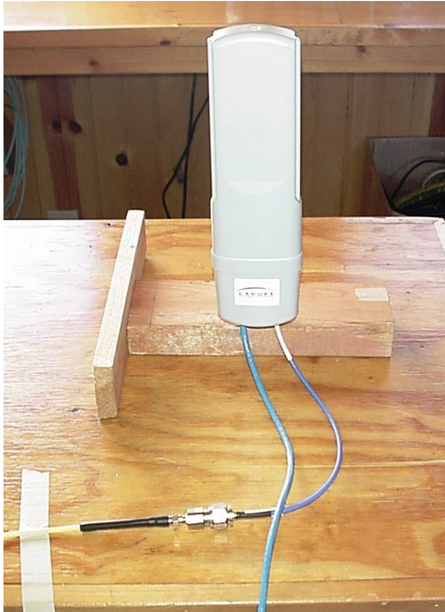
RF Conducted
