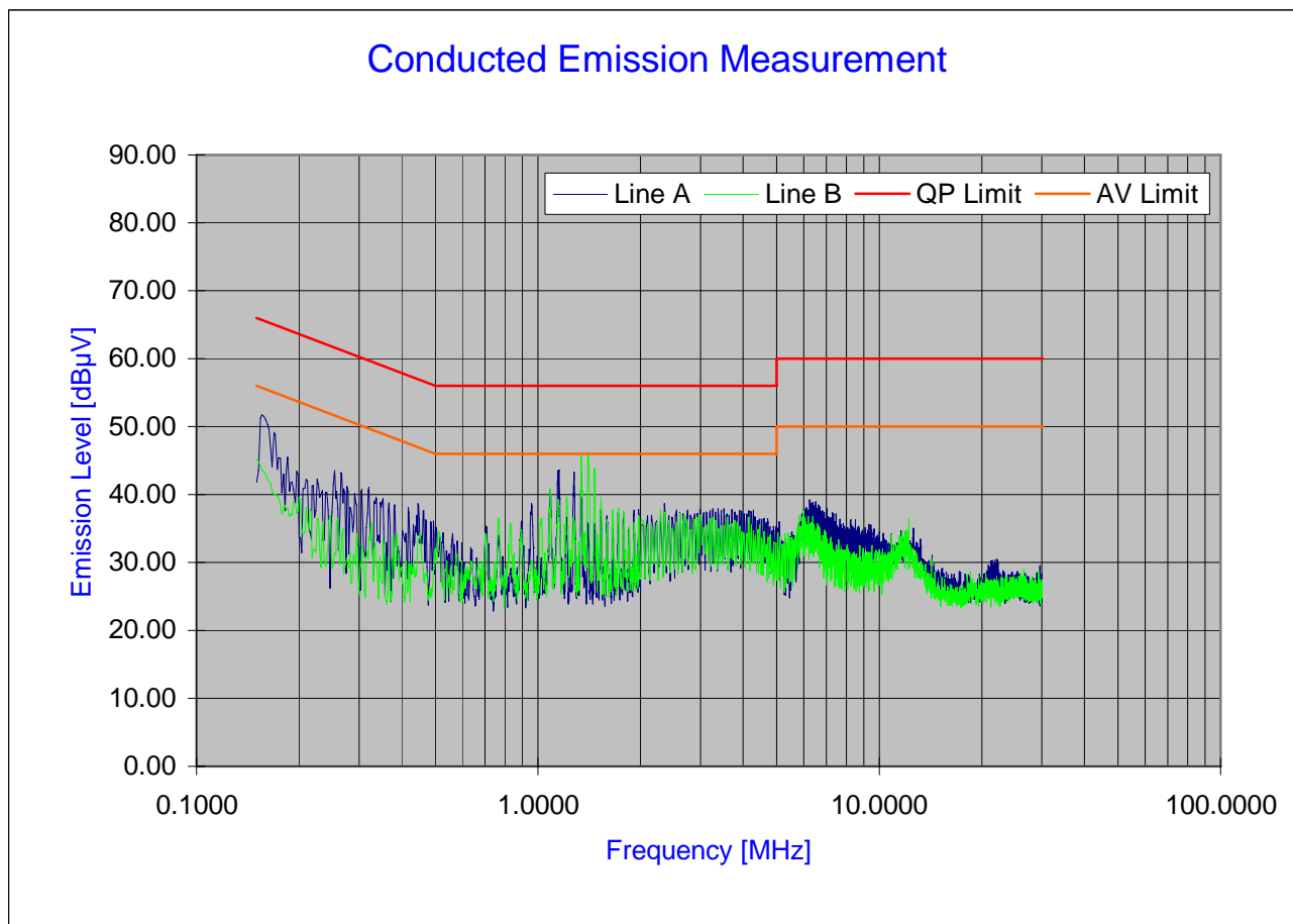
Plot 6-1. Line Conducted Plot for ML900 with 802.11a/b/g Module
