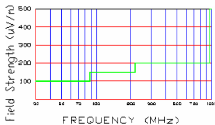
Figure 6-1. Radiated limits at 3 meters.
