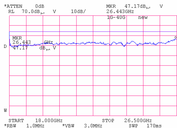
Plot 6.17.84: Tx Radiated emission measurements, 18 - 26.5GHz, at the mid carrier frequency, 802.11g mode.
