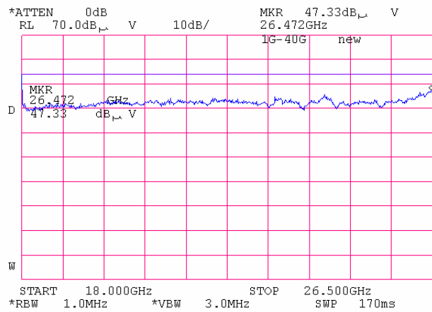
Plot 6.17.83: Tx Radiated emission measurements, 18 - 26.5GHz, at the low carrier frequency, 802.11g mode.
