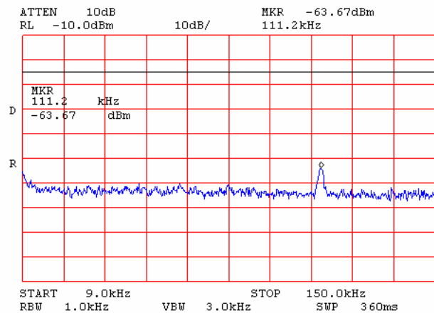
Plot 6.6.1: Tx Spurious emission measurements in 9 - 150 KHz range at low carrier frequency, OBW 5 MHz
