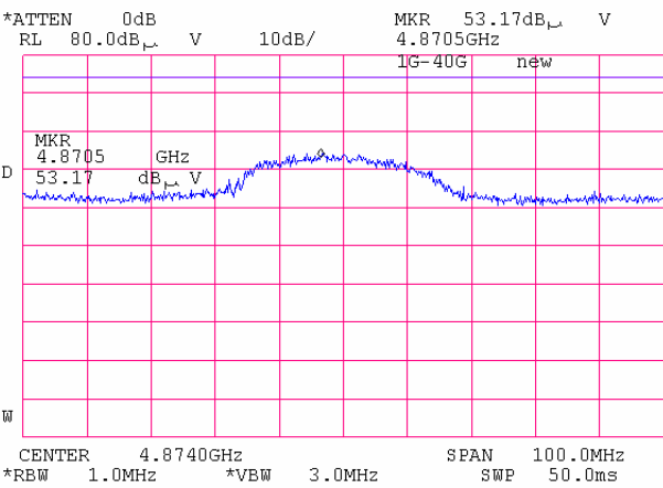
Plot 6.17.92: Tx Radiated emission measurement, at the 2 nd harmonic, at the mid carrier frequency, 802.11g mode.
