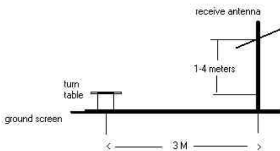
Figure 2. Diagram of 3-meter outdoor test range
