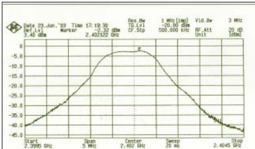
Channel 1 (2402MHz)
