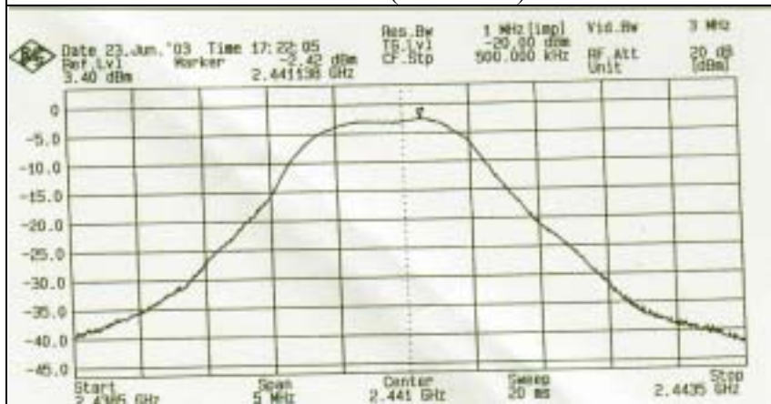
Channel 40 (2441MHz)
