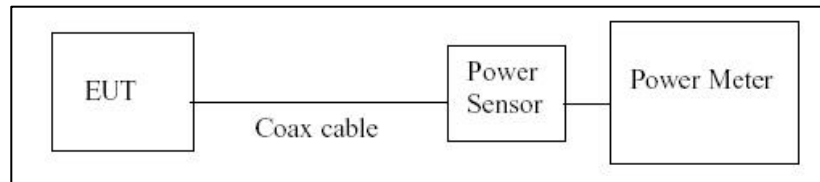
Figure A-2. Test Instrument & Measurement Setup
