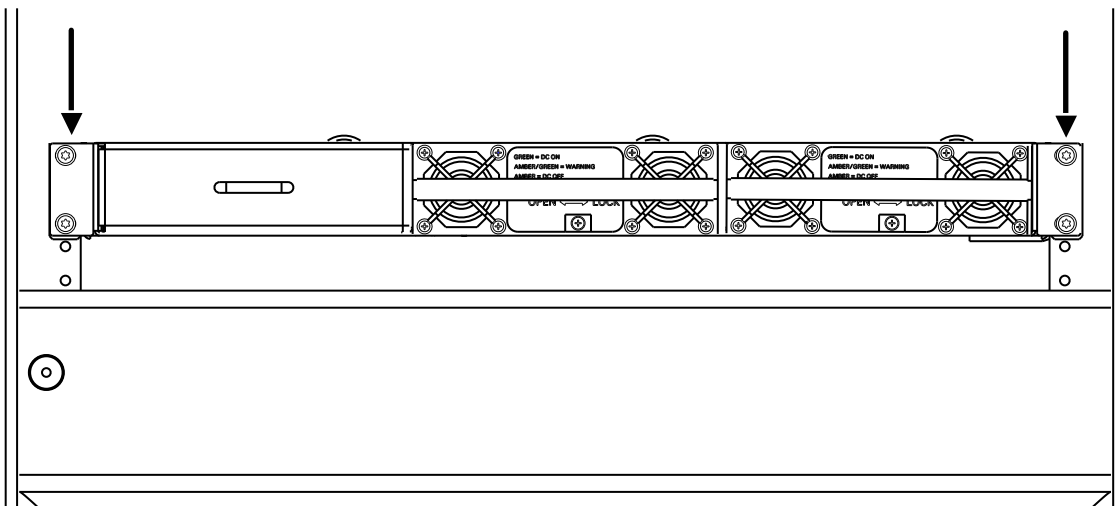
Figure 94: PSU Chassis Screws Location
