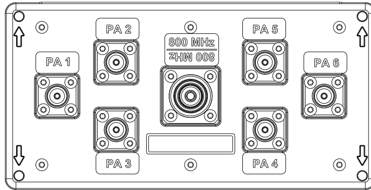
Figure 104: 4-6 N-Way Combiner
