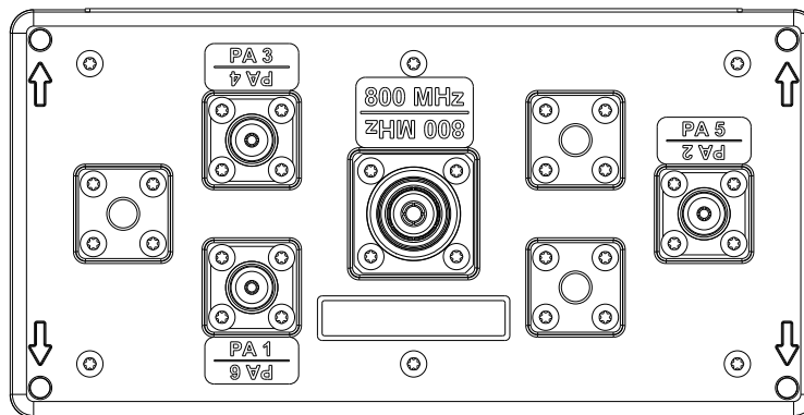
Figure 103: 2-3 N-Way Combiner
