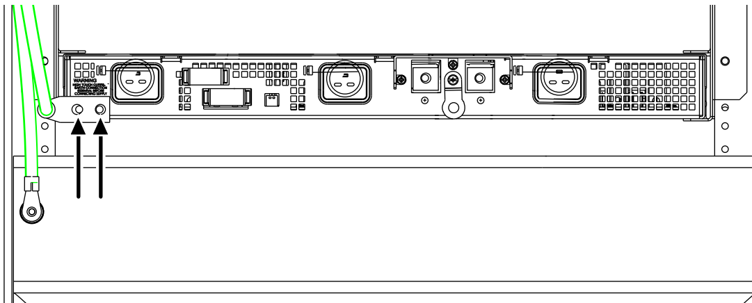
Figure 93: PSU Chassis Grounding Cable
