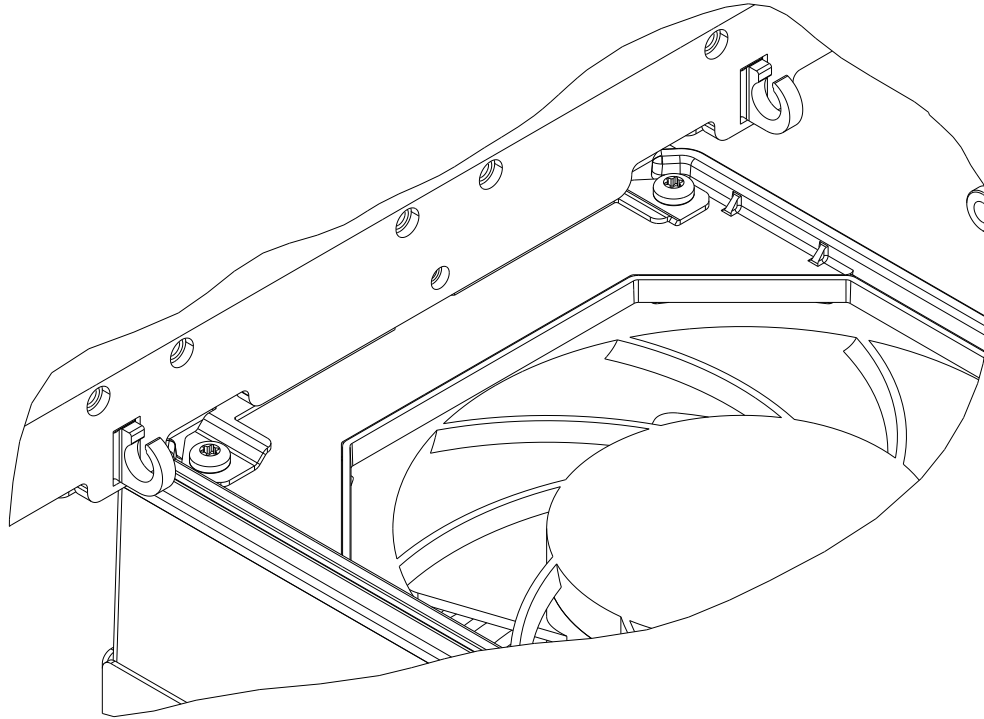
Figure 89: Fan Kit Retainer Lines and Card Cage Notch
