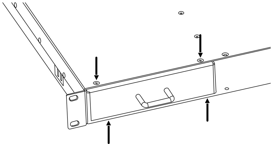
Figure 96: Retrieving the PSU Blank Panel
